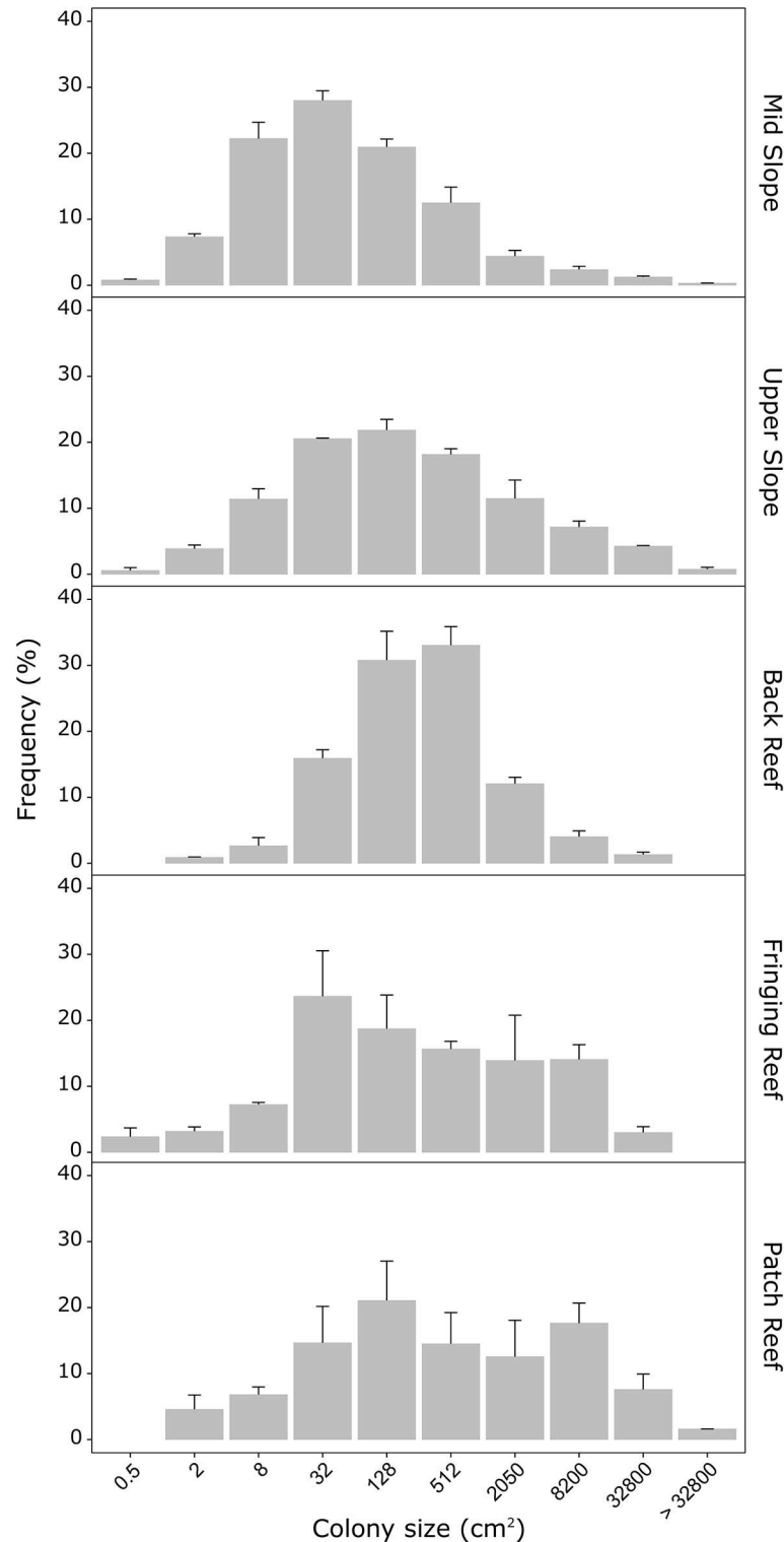
Fig 4. Size-frequency distributions of Millepora platyphylla across the five surveyed habitats. Colony size ( \text{cm}^2 ) data were distributed among 10 size classes based on a logarithm scale ( \log_2 ). Frequencies (%) for each size class were averaged by habitats with total population size (N in S2 Table) and error bars show the standard error for transect replicates.
