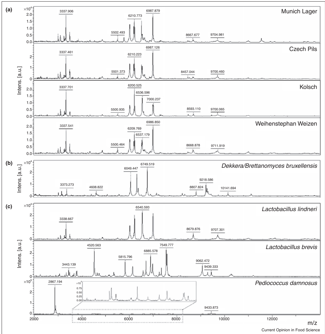
MALDI-TOF MS spectra of beer yeast and beer spoiling bacterial strains. (a) commercially available brewing yeasts, (b) wild yeast and (c) beer spoiling bacteria. The inset in Pediococcus damnosus spectrum represents an extension. (reprinted with permission from Springer).
