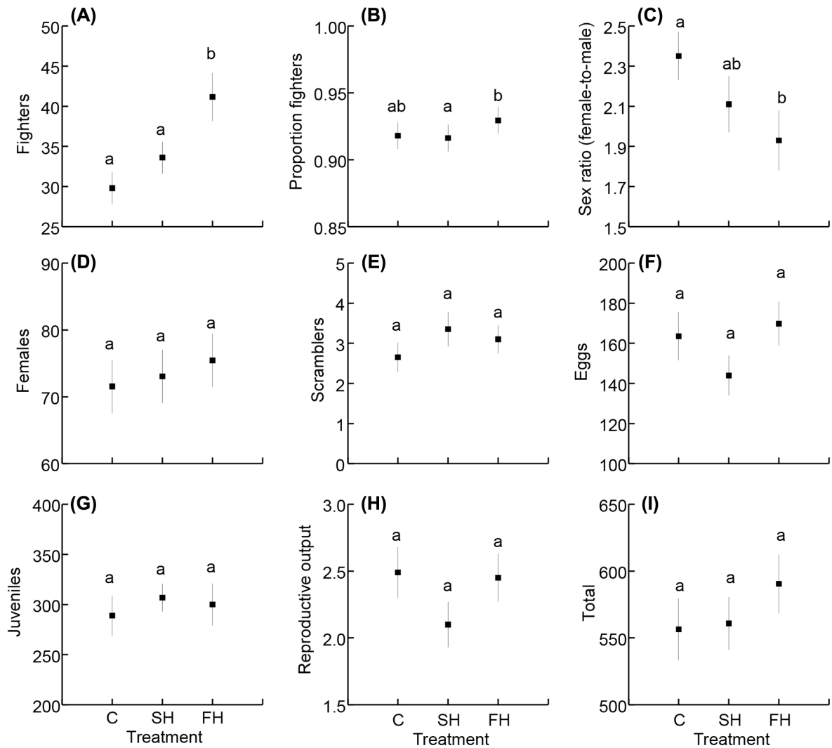
Figure 3. Mean number of fighters (A), proportion of males that were fighters (B), adult female-to-adult male sex ratio (C), number of adult females (D), number of scambler (E) number of eggs, (F), number of juveniles (G), reproductive output (number of eggs divided over the number of adult females) (H) and the mean total number of individuals (I) per treatment group, averaged over the experimental period (Fig. 2). C – control; SH – scambler harvesting; FH – fighter harvesting. The black squares are the observed means across replicate populations and the vertical lines are standard errors of the mean. Letters above the means in each panel denote whether treatments had a significant effect on each response variable at \alpha = 0.05 . Each treatment was replicated four times, resulting in 12 experimental populations, which structure and size was scored ten times over a period of 66 days.
