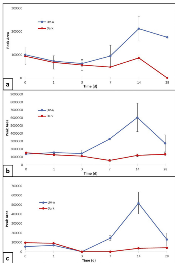
Fig. 3. Abundance (peak area) over time of (a) C60-I, (b) C60-II and (c) C60-III products in the glass incubation. The blue and red lines represent the irradiated (UV-A) and non-irradiated (Dark) samples, respectively. (For interpretation of the references to colour in this figure legend, the reader is referred to the web version of this article.)
