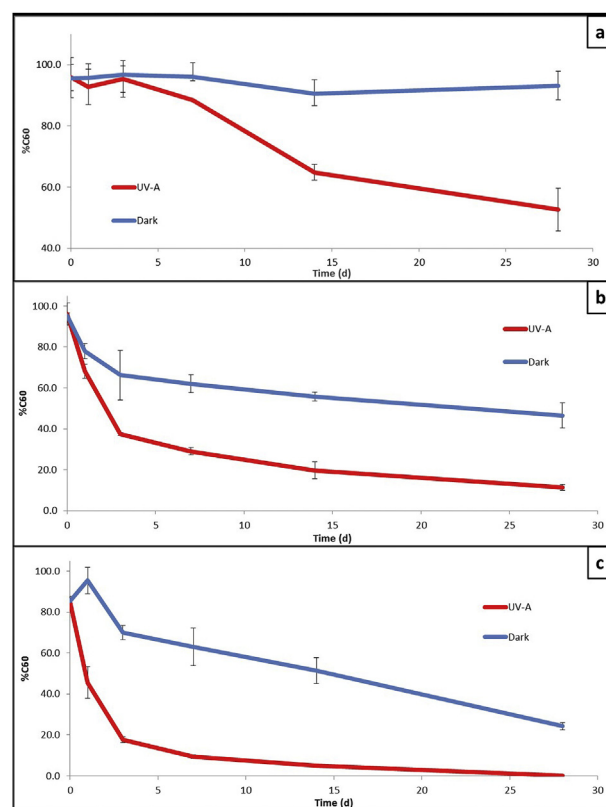
Fig. 1. Concentration of C_{60} fullerenes over time in (a) fullerenes dried on top of a glass surface ("glass"), (b) spiked into quartz sand and (c) spiked into sandy soil at the concentration of 100 \mu g/kg. The red line represents the sample irradiated with UV-A light whereas the blue line represents the samples incubated in the dark. (For interpretation of the references to colour in this figure legend, the reader is referred to the web version of this article.)
