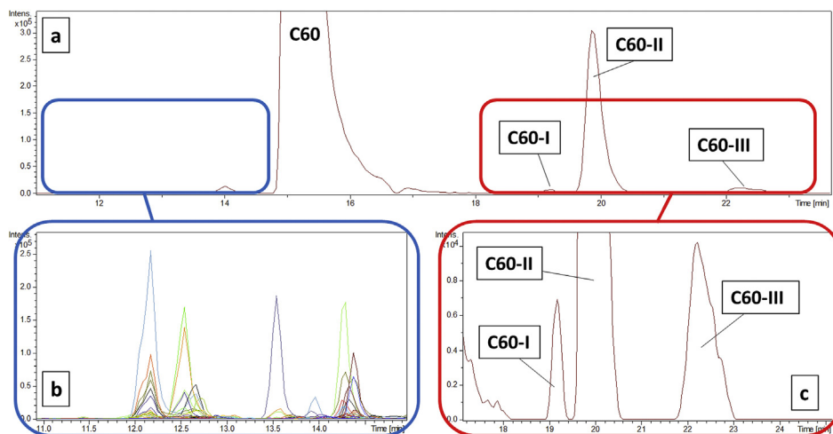
Fig. 2. UHPLC-HRMS analysis of glass incubation samples irradiated with UV-A light. (a) Chromatogram presenting the C_{60} peak at retention time 15 min and smaller C_{60} -containing peaks (C60-I, C60-II and C60-III) eluting later. (b) Several unknown peaks eluting before C_{60} (blue frame). (c) A zoom of the 18–24 min range (red frame), highlighting the presence of the C_{60} -containing ( C_{60} -like) structures. (For interpretation of the references to colour in this figure legend, the reader is referred to the web version of this article.)
