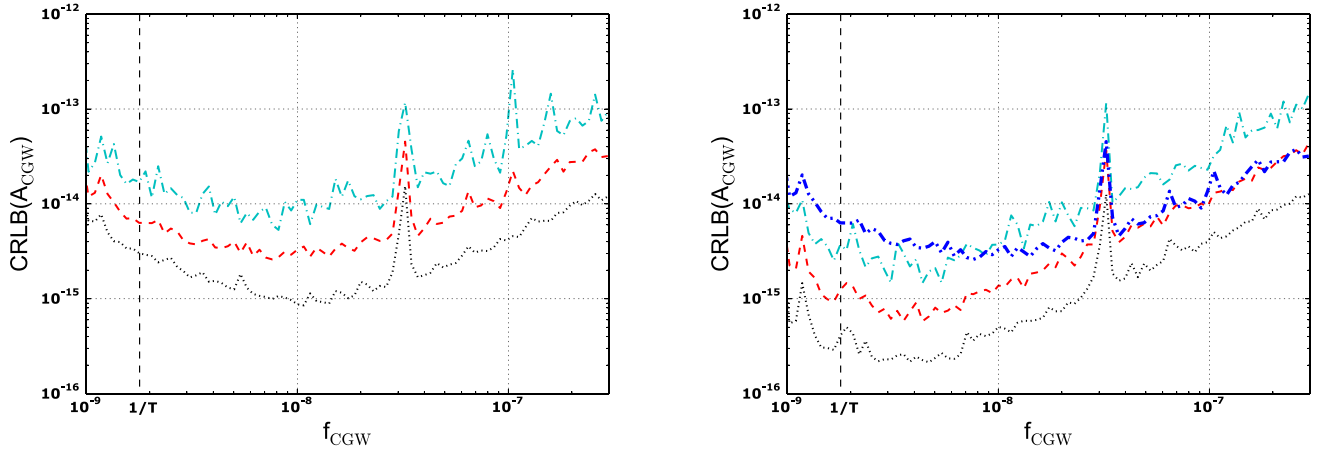
Figure 9. Results for the CRLB on the strain amplitude of CGWs, A_{\text{CGW}} , against the CGW frequency, f_{\text{CGW}} , from resolvable SMBHBs with circular orbits and without measurable frequency chirping. The different curves are for the cases where the SMBHB is at the sky location where the PTA has the maximum (cyan, dot–dashed lines) and minimum (black, dotted lines) sensitivity, and the average of all positions on the sky (red, solid lines). The vertical line show the frequency resolution of the PTA, 1/T , where T is time-span of the pulsar with the longest data set. Left-hand panel: sensitivity curves when accounting for the white and the TN of the data. Right-hand panel: sensitivity curves when only accounting the white noise of the data. The additional blue, thick double dot–dashed line is the case for mean PTA sensitivity when including the TN as in the left-hand panel (red, solid line) for better comparison.
