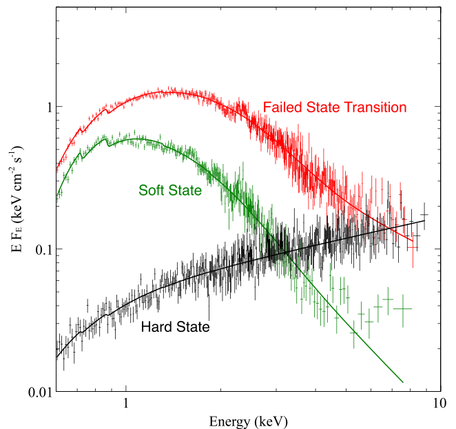
Figure 3. A comparison of unfolded Swift -XRT spectra from three epochs: during the failed state transition (2012 April 24; red), during the hard state (2013 June 18; black) and during the apparent new accretion state (2015 March 17; green). The 2012 and 2015 data are fitted with DISKBB+POWERLAW and the 2013 data are fitted with POWERLAW (solid lines).
