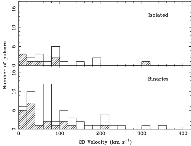
Figure 5. Histogram of the 2D velocity distribution for a sample of 19 isolated MSPs (top panel) and 57 binary MSPs (bottom panel). The respective average velocities are 88 \pm 17 and 96 \pm 12 \text{km s}^{-1} . The hatched part of the histogram shows the pulsars with a distance estimate from the parallax measurement (eight isolated and 21 binary MSPs).
