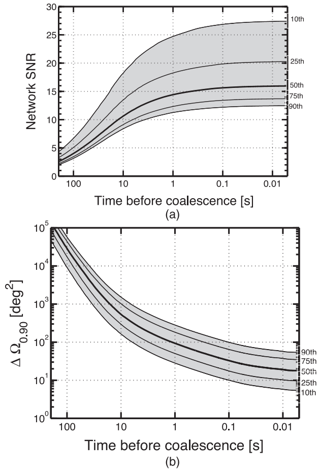
Figure 3. Percentile curves of (a) network SNR and (b) \Delta\Omega (error box at 90 per cent confidential level) as a function of time before merger for the simulated BNS triggers obtained by an LHV network.
