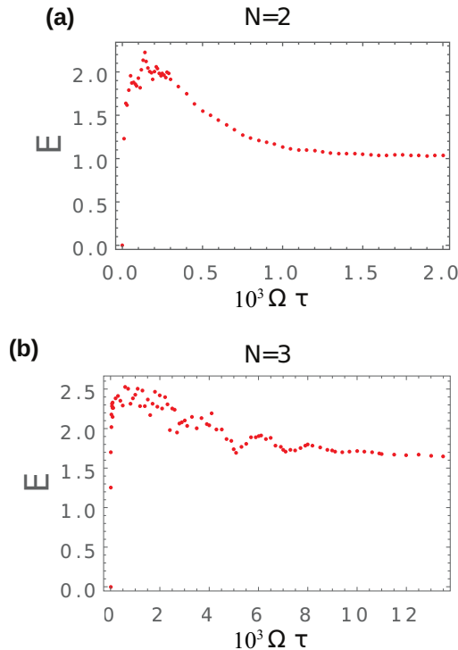
FIG. 5. Entanglement, as measured by the logarithmic negativity, for different pulse amplitudes and (a) N = 2 , (b) N = 3 . Parameters used are \Delta t/\tau = 0.36 , \Omega_r^{\max} = \Omega_e^{\max} = \Omega , and U\tau/\hbar = 2\Omega .
