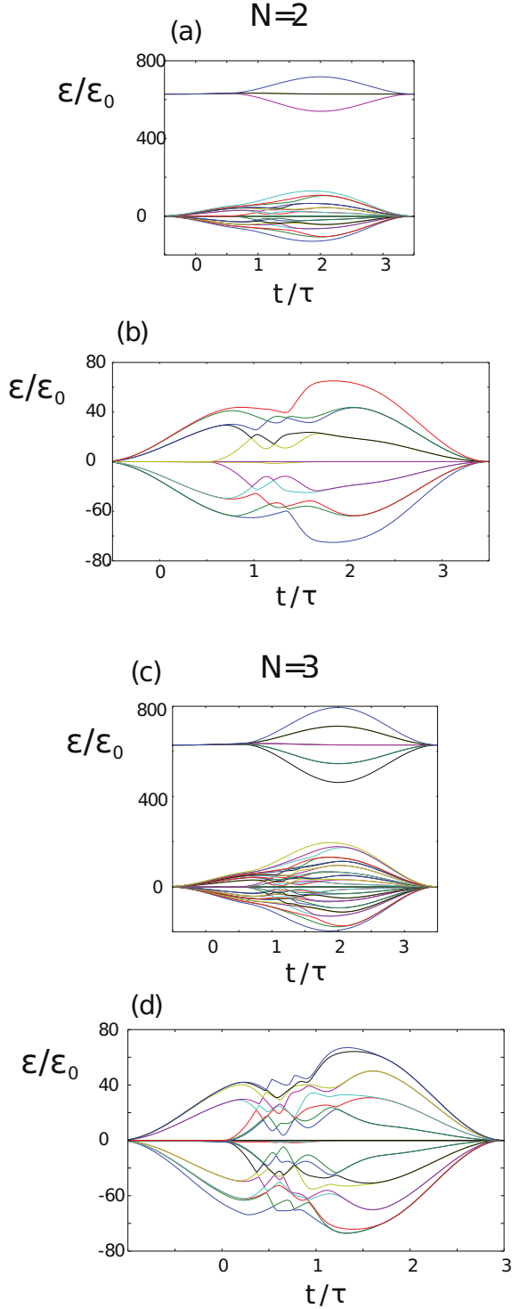
FIG. 2. Energy eigenvalues \varepsilon of the Hamiltonian Eq. (15) for (a, b) N_1 = N_2 = 2 and (c, d) N_1 = N_2 = 3 . (b) and (d) are zoomed in versions of (a) and (c) near the zero-energy region. We use pulses for \Omega_{e,r} as defined in Eqs. (30) and (31). Parameters used are \epsilon_0 = \hbar/\tau , \Delta t/\tau = 0.11 , \Omega_r^{\max}\tau = 500\pi , \Omega_e^{\max}\tau = 500\pi , and U\tau/\hbar = 200\pi .
