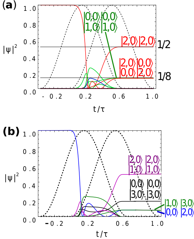
FIG. 3. Probability amplitude |\psi_n|^2 evolution during the STIRAP sequence for states |k_1, k_2, r_1, r_2\rangle with (a) N = 2 and (b) N = 3 . In (a), horizontal lines show populations of labeled states in the ideal adiabatic case. Parameters used are (a) \Delta t/\tau = 0.36 , \Omega_r^{\max}\tau = 60\pi , \Omega_e^{\max}\tau = 60\pi , U\tau/\hbar = 200\pi ; (b) \Delta t/\tau = 0.36 , \Omega_r^{\max}\tau = 10^4 , \Omega_e^{\max}\tau = 10^4 , U\tau/\hbar = 2\Omega_r^{\max} .
