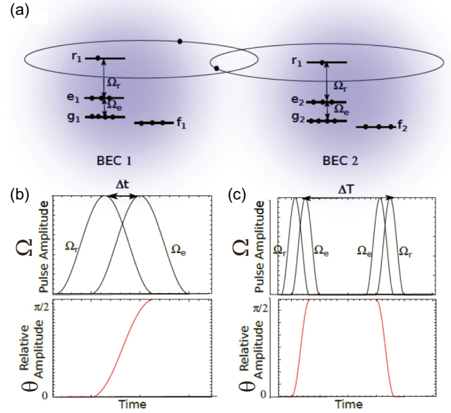
FIG. 1. (a) Representation of the energy levels used for the STIRAP schemes. g_i and f_i are the energy levels of the ground states of the atoms forming the BECs for i = 1, 2 . e_i are the energy levels for the excited states, and r_i are the Rydberg levels. (b) Pulses for the STIRAP sequence. The pulses are in counterintuitive order: the sequence starts with the pulse coupling the unpopulated states |e_i\rangle and |r_i\rangle , not affecting the initial state until the pulse coupling the states |e_i\rangle and |g_i\rangle is turned on. (c) Pulses for the two-STIRAP sequences. The second pulse sequence is in reverse order compared to the first one. The relative amplitude \tan \theta = |\frac{\Omega_e}{\Omega_r}| is also plotted for the one- and two-STIRAP sequences.
