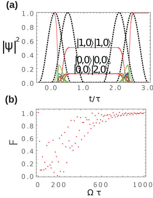
FIG. 6. (a) Typical time evolution for the geometric phase gate with two STIRAP sequences for N_1 = N_2 = 2 from the initial state |k_1 = 0, r_1 = 0\rangle |k_2 = 0, r_2 = 0\rangle . Parameters used are \Delta t/\tau = 0.40 , \Omega_r^{\max} \tau = 1000 , \Omega_e^{\max} \tau = 1000 , U\tau/\hbar = 2\Omega_e^{\max} , \omega\tau = -0.05 , and \Delta T/\tau = 2 . (b) Fidelity of the initial state after the two STIRAP pulses for various values of \Omega_r^{\max} = \Omega_e^{\max} = \Omega .
