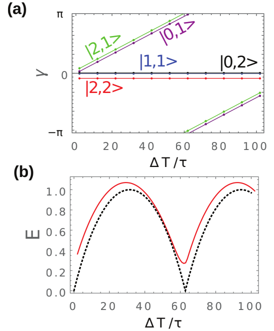
FIG. 7. (a) Phases picked up during two STIRAP pulse procedure by various states as labeled by |k_1, k_2\rangle = |k_1, 0, 0\rangle_z |k_2, 0, 0\rangle_z in Eq. (49). The phases picked up by |k_2, k_1\rangle are the same as |k_1, k_2\rangle . Parameters used are the same as in Fig. 6(a). Phases are with references to the state |0, 0\rangle , which does not pick up any phase under the evolution. (b) Entanglement created by evolving the two STIRAP sequence starting from the state |\frac{1}{\sqrt{2}}, \frac{1}{\sqrt{2}}\rangle |\frac{1}{\sqrt{2}}, \frac{1}{\sqrt{2}}\rangle . Solid line shows the result for the phases picked up as in subfigure (a). Dashed lines shows the ideal result Eq. (60).
