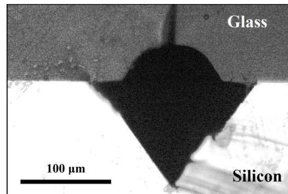
Figure 3. Microchannel in SOG ship after silicon wet etching by KOH solution
