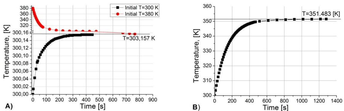
Figure 7. Maximum chip temperature change over time. (A) F_{ch}=10^{-6} [m 2 ], (B) F_{ch}=10^{-4} [m 2 ]
