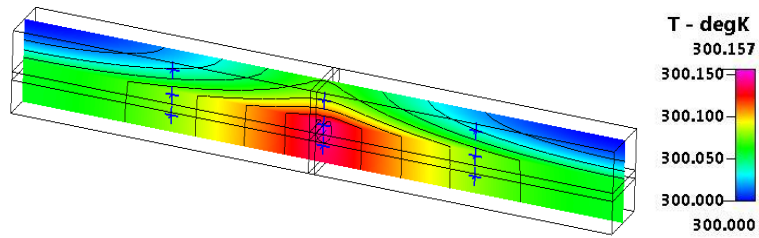
Figure 6. Temperature distribution in cross-section of chip ( F_{ch}=10^{-6} [m 2 ], R=10^{-12} [m 3 /s])
