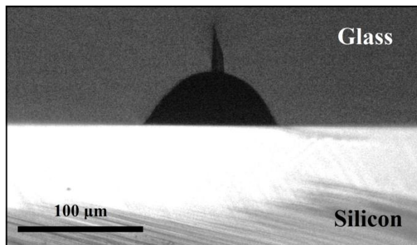
Figure 2. Microchannel in SOG ship before silicon etching
