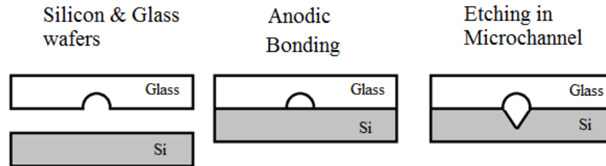
Figure 1. Scheme of etching-in-microchannel technology
