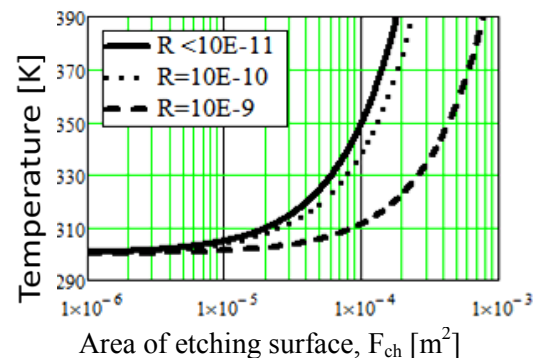
Figure 8. Equilibrium temperature of the chip. Analytical model
