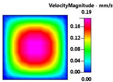
Figure 5. Velocity in microchannel ( R=10^{-12} [m 3 /s])
