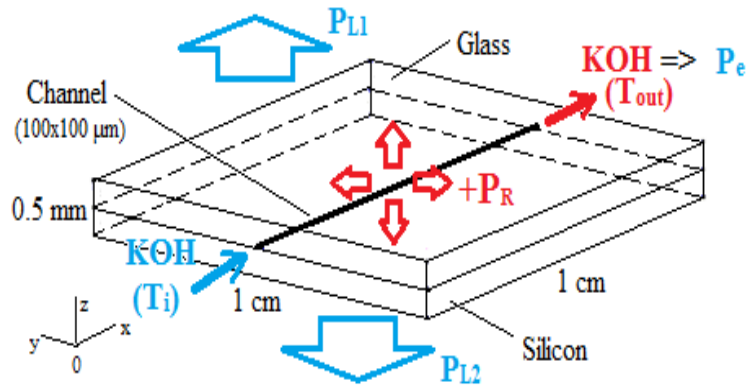
Figure 4. Scheme of SOG chip with microchannel
