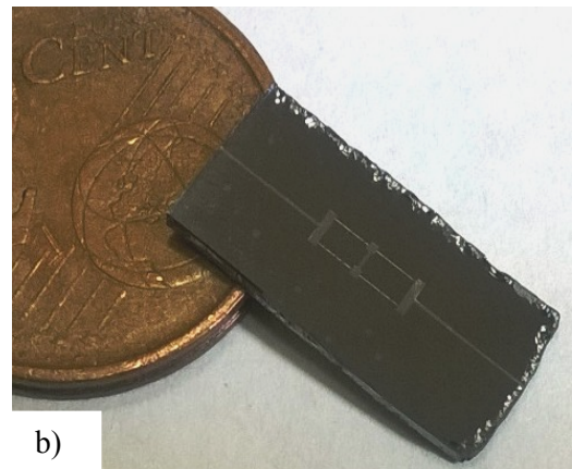
Figure 2b. Silicon-glass prototype of the microfluidic Wheatstone bridge.
