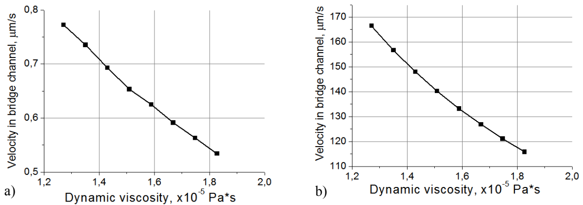
Figure 6. Velocity in the bridge microchannel for different viscosity of fluid and \Delta P_{MWB} = 5000 Pa. a) Width of “X” channel is 36.4 \mu\text{m} (near balance configuration); b) Width of “X” channel is 40 \mu\text{m} .
