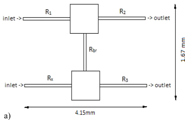
Figure 2a. Scheme of the microfluidic Wheatstone bridge.
