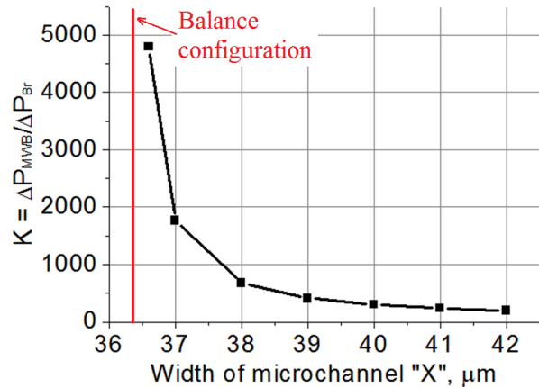
Figure 8 Pressure reduction coefficients for different width of the microchannel “X”.
