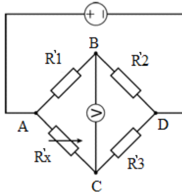
Figure 1. Electric circuit of the Wheatstone bridge.
