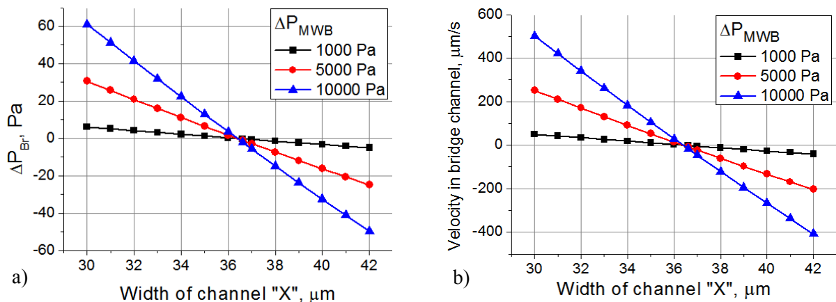
Figure 5. Pressure drop (a) and velocity (b) in the bridge microchannel for different width of the channel R_X and pressure in the MWB. Viscosity is 1.58910^{-5} \text{ Pa}\cdot\text{s}
