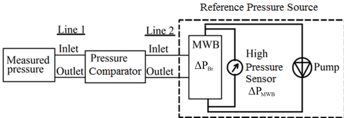
Figure 9. Architecture of the high accuracy microfluidic pressure sensor based on the MWB.
