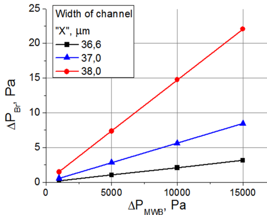
Figure 7 \Delta P_{Br} as a function of \Delta P_{MWB} for different width of channel “X”.
