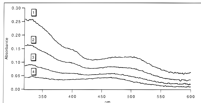
Figure 3. Transient absorption spectrum of [ 4 :8]- anti in benzene (1) just after, (2) 25 ns after, (3) 50 ns after, and (4) about 100 ns after the laser pulse. The decay at 490 nm (as that at 350 nm) can be fitted to a monoexponential decay of 53 ns. The long-lived component is due to the absorption of the triplet state which has an infinite lifetime on this time scale.
