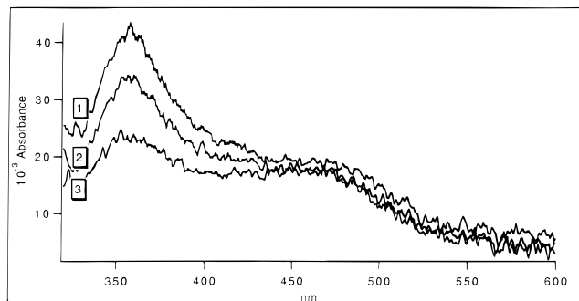
Figure 5. Transient absorption spectrum of [ 4 :8]- anti in THF (1) just after, (2) 4 ns after, and (3) 8 ns after the laser pulse. The decay at 490 nm is too fast (<5 ns) to be fitted. On longer time scale, a long-lived component with an absorption at 470 nm remains which is due to the absorption of the triplet state and has an infinite lifetime on this time scale. Because of spectral overlap, it is left out for clarity.
