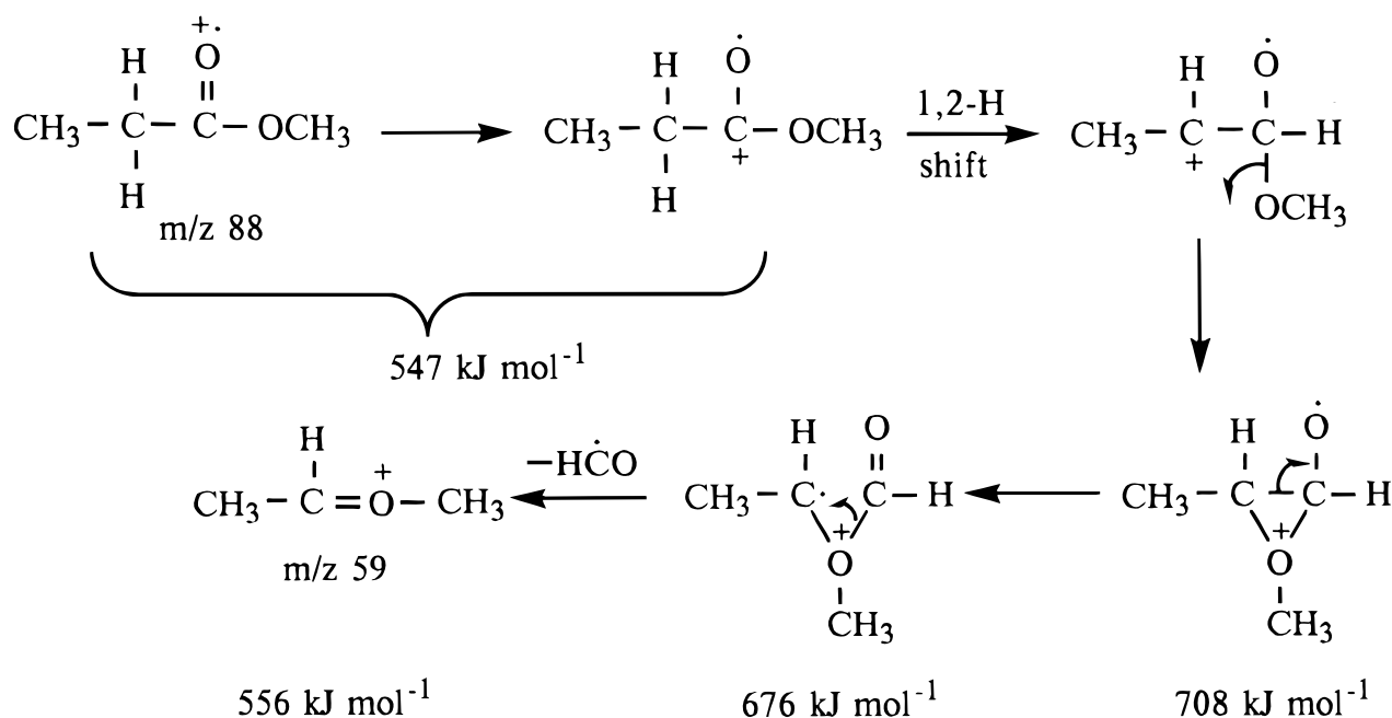
Scheme 1. Mechanism proposed for the loss of H\dot{C}O from the molecular ion of methyl propanoate (1). The values given under the structures are the heats of formation calculated at the ROHF/6-31G* level of theory 16 with reference to the heat of formation of 1^+ ( 547 \text{ kJ mol}^{-1} ). 14 For the top-right structure no stable energy minimum has been obtained. The value of 556 \text{ kJ mol}^{-1} for the bottom-left structure was taken from Ref. 15.
