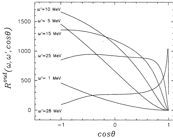
Fig. 1. The scattering rate R^{out}(\omega, \omega', \cos\theta) (in arbitrary units) at fixed neutrino energy \omega = 30 MeV and six different \omega' energies: 1, 5, 10, 15, 25 and 28 MeV. The neutrino energies \omega' are indicated in the figure. The electrons are taken at a temperature T = 1.6 MeV and degeneracy \xi_e = 17 (dimensionless).
