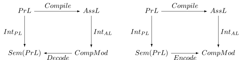
Figure 1: Compiler correctness.
