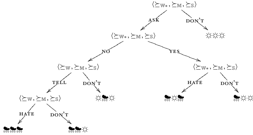
Figure 4: The description tree t \mapsto S(t, \mathbb{M}) = S_{\mathbb{M}}(t, \emptyset) of Mary's beliefs. This is also the description tree of S_{M^W} and S_{M^{WW}} .
