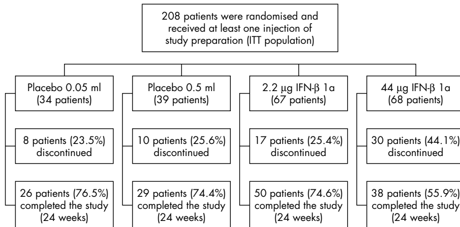
Figure 1 Patient disposition.
