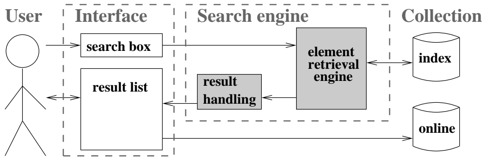
Figure 8.1: Simplified image of the interaction taking place when a user interacts with our focused retrieval system via our interface.
