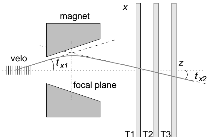
Figure 3.2: A deflected track in the x - z plane. t_{x_1} is the angle with the z -axis in the VELO, t_{x_2} the angle at the tracker stations T1, T2 and T3. The deflection in the magnetic field is modelled as if the track kinks at the focal plane of the magnet.
