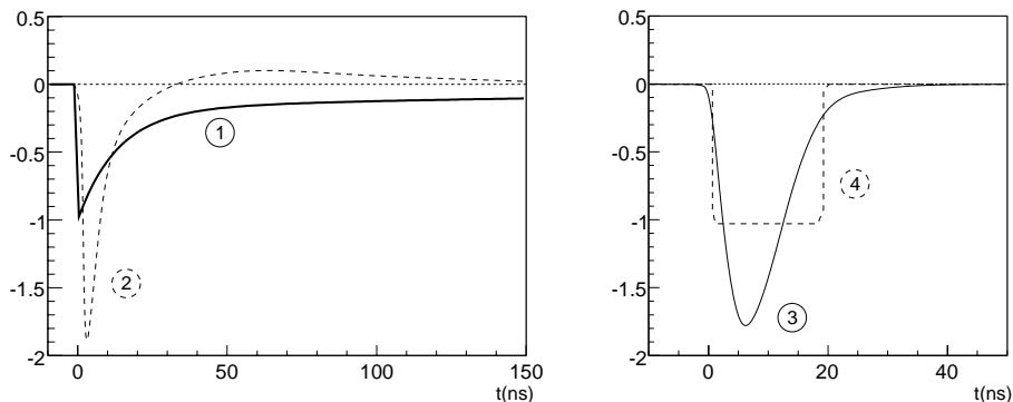
Figure 4.8: Illustration of the signal shapes versus time t in ns after the ASDBLR stages. In the left graph, the preamplifier (1) and shaper output (2) are drawn. In the right graph, (3) is the signal after the baseline restoration and curve (4) represents the discriminator output.
