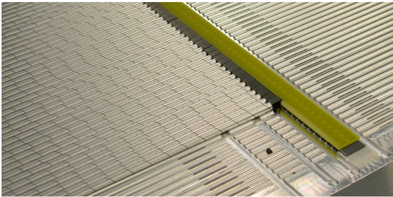
Figure 3.19: Photograph of straw tubes in the jig at the straw tube separation zone halfway the module. The straws, endpieces and pc-boards can be seen at the picture; a cross-section of the assembly is sketched in Fig. 3.18.
