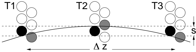
Figure 5.5: Sketch of a deflected track (solid line) which is reconstructed as a straight line in the region of the tracker stations. The maximum sagitta s over the distance \Delta z between T1 and T3 equals the channel pitch. Channels which are hit by the particle are shaded: hit channels compatible with both the curved and a straight track are filled.
