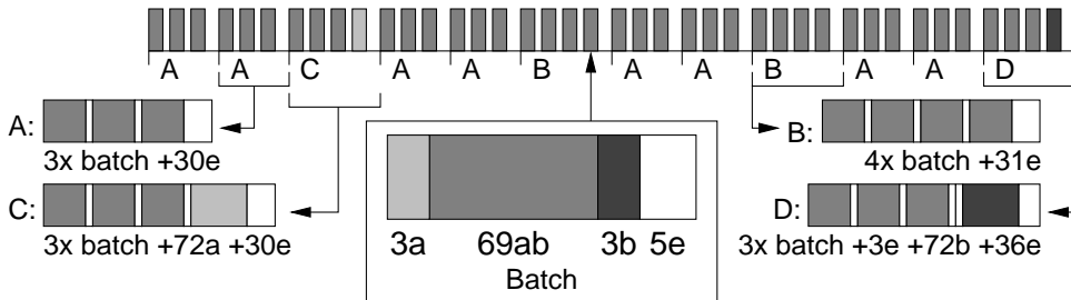
Figure 2.2: LHC bunch structure for one revolution at the IP8 interaction point. Bunch crossings can have two filled (ab) or empty (e) bunches, as well as one filled and one empty bunch (a,b).
