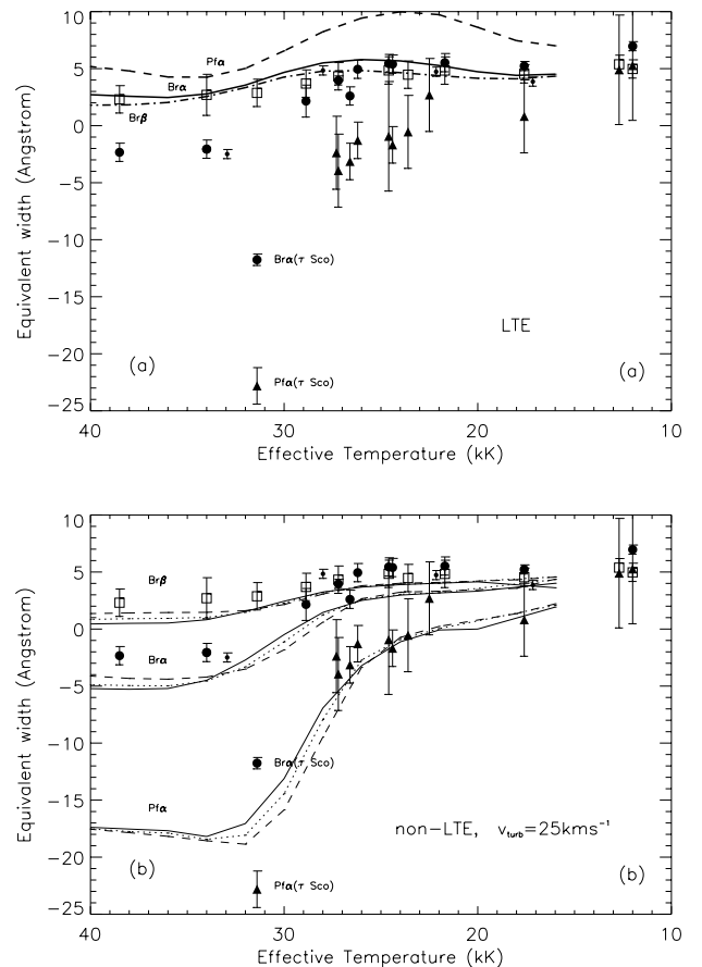
Fig. 6. a) Comparison between observed equivalent widths for \text{Br}\alpha (solid), \text{Br}\beta (dot-dashed) and \text{P}\text{f}\alpha (dashed) and predicted values assuming LTE and v_{\text{turb}} = 0 \text{ km s}^{-1} , and b) assuming non-LTE and v_{\text{turb}} = 25 \text{ km s}^{-1} . For the LTE models we only used \log g = 4.0 . In the case of non-LTE models the same gravity values (and linestyles) are used as in Fig. 4
