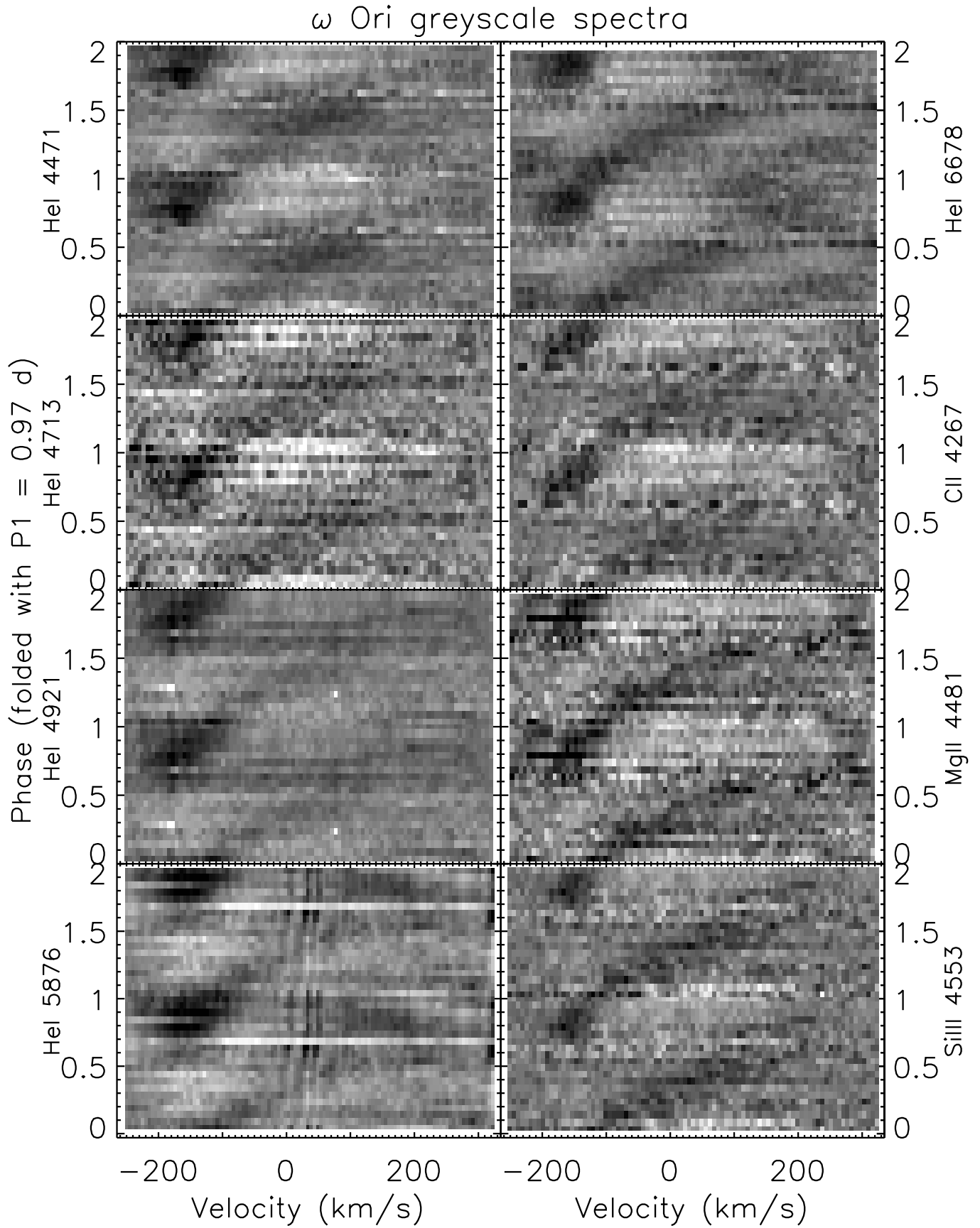
Fig. 16. The greyscale plots of all spectra for each studied line normalized by its mean profile folded in phase with the frequency f_1 = 1.03 \text{cd}^{-1} . The velocity range corresponds to the one determined by the variance of He I lines.
