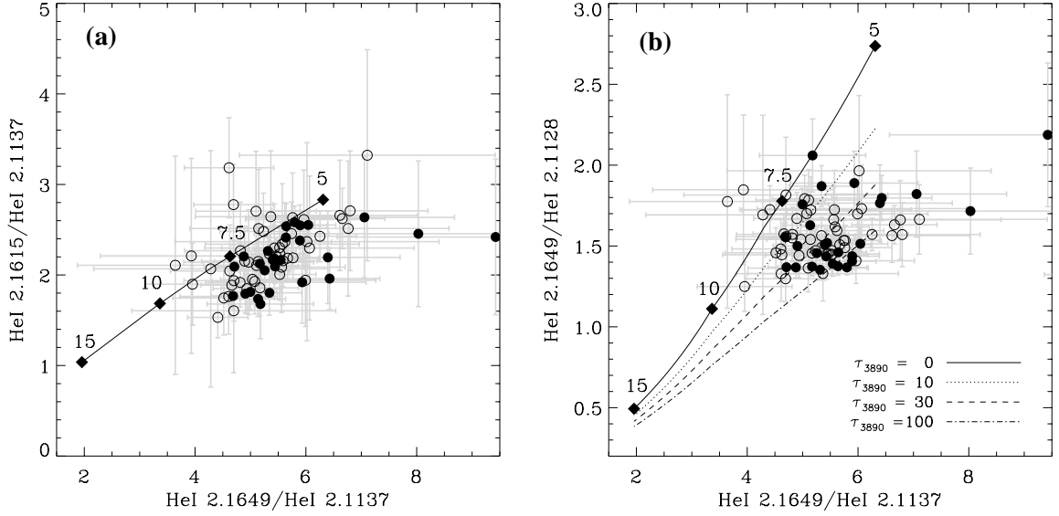
Fig. 7. a) Plot of the line ratio 2.1615\text{-}7^3\text{F-}4^3\text{D}/2.1137\text{-}4^1\text{S-}3^1\text{P} against the ratio 2.1649\text{-}7^{1.3}\text{G-}4^{1.3}\text{F}/2.1137\text{-}4^1\text{S-}3^1\text{P} . Note that these line ratios should not depend on radiative transfer effects. b) 2.1649\text{-}7^{1.3}\text{G-}4^{1.3}\text{F}/2.1128\text{-}4^3\text{S-}3^3\text{P} against 2.1649\text{-}7^{1.3}\text{G-}4^{1.3}\text{F}/2.1138\text{-}4^1\text{S-}3^1\text{P} . In both figures, the solid line represents the Case B predictions for T_e = 5, 7.5, 10 and 15 \times 10^3 K (indicated by solid diamonds) and n_e = 10^4 \text{ cm}^{-3} . The data indicate a temperature between 5000 and 7500 K. The non-solid lines in b) represent the calculations by Benjamin et al. (2002) for non-zero optical depth of the 2^3\text{S} metastable level. Only points located in the interval [-5'', +8''] are considered. The data points from the tail of G29.96 ( >0'' ) are plotted as open circles; those from the arc ( <0'' ) are plotted as solid circles. The open and filled circles have very similar distributions.
