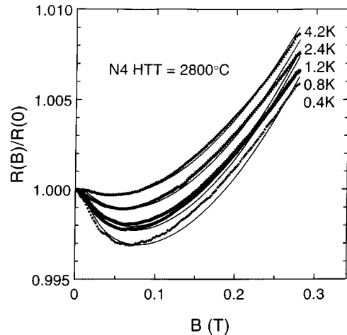
FIG. 9. Magnetoresistance, normalized at B=0 , versus magnetic field for sample N4 (HTT=2800 °C) at temperatures between 0.4 and 4.2 K as indicated. The various symbols represent the data points. The solid lines represent the best fit to Eq. (8).
