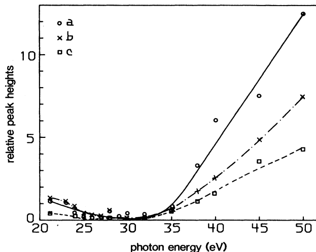
FIG. 13. Intensity (peak height) as a function of photon energy of the main peaks in the normal emission spectra of \text{SnTaS}_2 , relative to the intensity of the lowest-lying S\ 3p peak at 6 eV binding energy. (a) Peak at binding energy 1 eV ( \text{Ta}\ 5d_{z^2} ); (b) peak at binding energy 2.3 eV; (c) peak at binding energy 2.9 eV.
