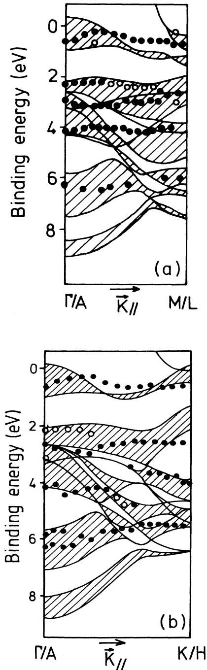
FIG. 11. Comparison of experimental and calculated band structure of SnTaS 2 in the (a) \Gamma M L A plane and (b) the \Gamma K H A plane.
