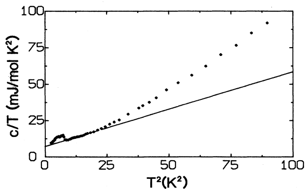
FIG. 18. C/T vs T^2 of \text{SnTaS}_2 .
