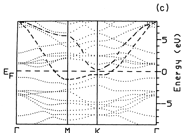
FIG. 6. The calculated Sn 5 p x,y band. (a) Tight-binding method: density of states. (b) Tight-binding method: energy-dispersion curves along \Gamma MK\Gamma . (c) ASW method; dotted and dashed curves are ASW calculated energy bands. The dashed curves are bands with mainly Sn 5 p x,y character.
