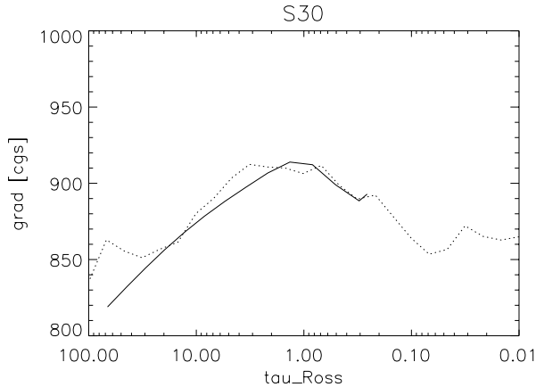
Fig. 11. Comparison of total photospheric radiative acceleration for model S30 (bold) vs. results from an analogous hydrostatic Kurucz-model (dotted). Note that the gravitational acceleration for this model is 1000 \text{ cm s}^{-2} , i.e., the radiative acceleration is very close to this value and, thus, of extreme importance (cf. Fig. 10). The deviations at largest depths are due to the fact that this model becomes (spherically) extended in the lowermost photosphere, an effect which cannot be treated in a plane-parallel approach (cf. Paper I).
