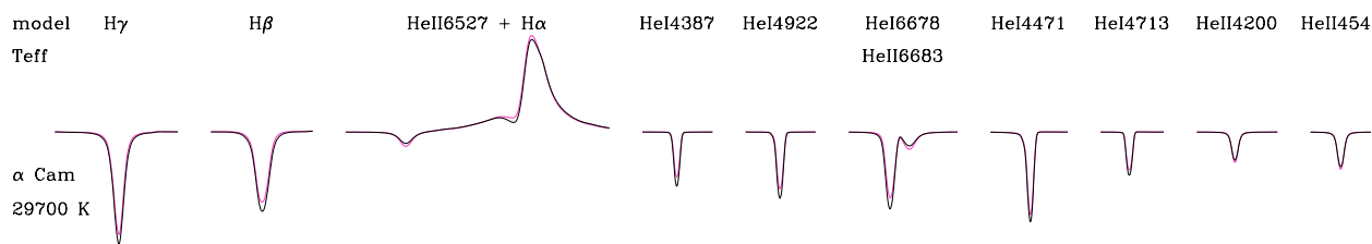
Fig. 18. Wind-strength parameter Q as an optical depth invariant: H/He profiles for the model of \alpha Cam as determined by Repolust et al. (2004), with \dot{M} = 6.04 \times 10^{-6} M_{\odot}/\text{yr} and R_{\star} = 32.5 M_{\odot} . Overplotted in magenta are the corresponding profiles for a model with identical Q -parameter (Eq. (93)) but different mass-loss rate and radius ( \dot{M} = 3.3 \times 10^{-6} M_{\odot}/\text{yr} and R_{\star} = 21.7 M_{\odot} ).
