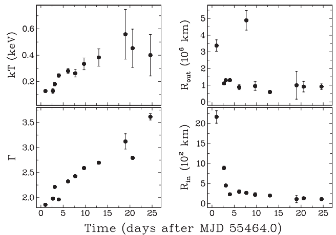
Figure 5. Evolution of the disc temperature (top left), photon index of the Compton tail (bottom left), outer disc radius (top right) and inner disc radius (bottom right). These parameters are based on spectral fits to the broad-band SEDs indicated in Fig. 1, using the irradiated disc model.
