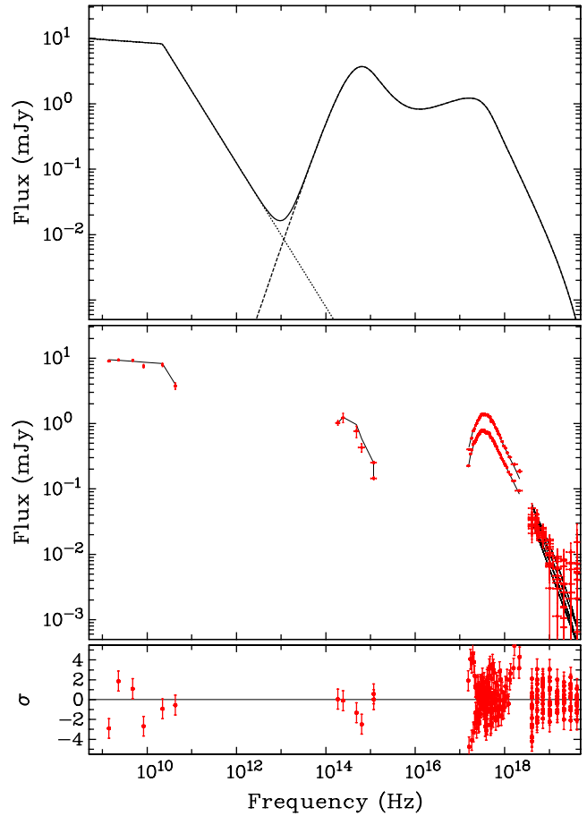
Figure 4. Example model plots for the broad-band SED at day 8 after the outburst onset. The top panel shows the spectrum of the best-fitting model for this particular epoch, with the dotted line showing the broken power-law fit to the radio data, the dashed line the irradiated disc model fit and the solid line the total spectrum. The middle panel shows the fit of the unfolded spectrum, with the data in red symbols and the best-fitting model in black lines. In the bottom panel we show the deviations from the best-fitting model.
