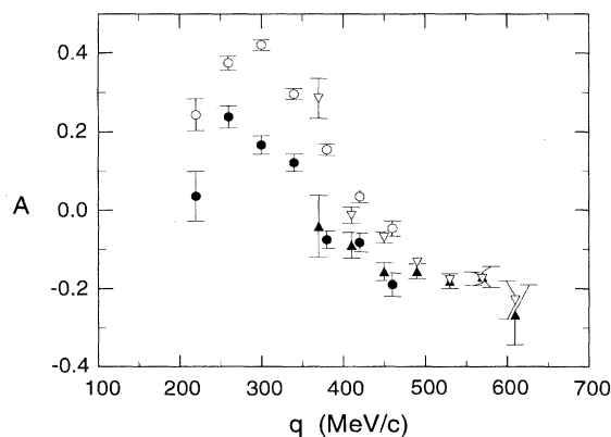
FIG. 2. The target (filled symbols) and beam (open symbols) analyzing powers, A_{00n0}^{3,n} and A_{000n}^{3,n} , respectively, for {}^3\text{He}(p, pn) at |p_m| > 100 MeV/c as a function of the 3-momentum transfer to the struck neutron |\mathbf{q}| . Data where the proton scattered to the right (left) detector and neutrons to the left (right) detector are indicated by circular (triangular) symbols.
