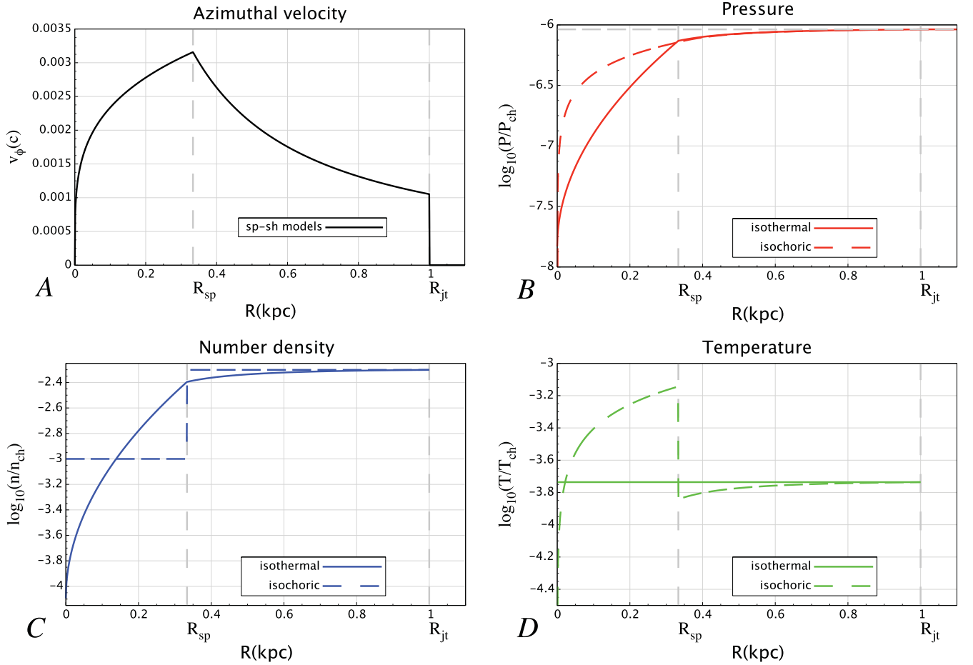
Figure 9. Initial transverse jet profiles for the isothermal jet (solid lines) and the piecewise isochoric jet (dashed lines), but now in the case of V_{\phi} = V_{\phi,C}^A = 3.159 \times 10^{-3}c . The cross-cuts show in black the profile of azimuthal rotation v_{\phi}(R) (panel A). This rotation profile has been used for both the isothermal and the isochoric jet model; in red , the \log_{10} of the pressure P in units of the characteristic pressure P_{\text{ch}} = 1.50 \times 10^{-6} \text{ erg cm}^{-3} (panel B); in blue , the \log_{10} of the number density n in units of the characteristic number density n_{\text{ch}} = 10^{-3} \text{ cm}^{-3} (panel C); and in green , the \log_{10} of the thermal temperature T in units of the characteristic temperature T_{\text{ch}} = 1.09 \times 10^{13} \text{ K} (panel D) of the jet. In addition, the images show the jet radius at R_{\text{jt}} = 1 \text{ kpc} and the jet spine radius at R_{\text{sp}} = R_{\text{jt}}/3 as the two vertical dashed lines. The pressure of the ambient medium is denoted by the dashed horizontal line in panel B.
