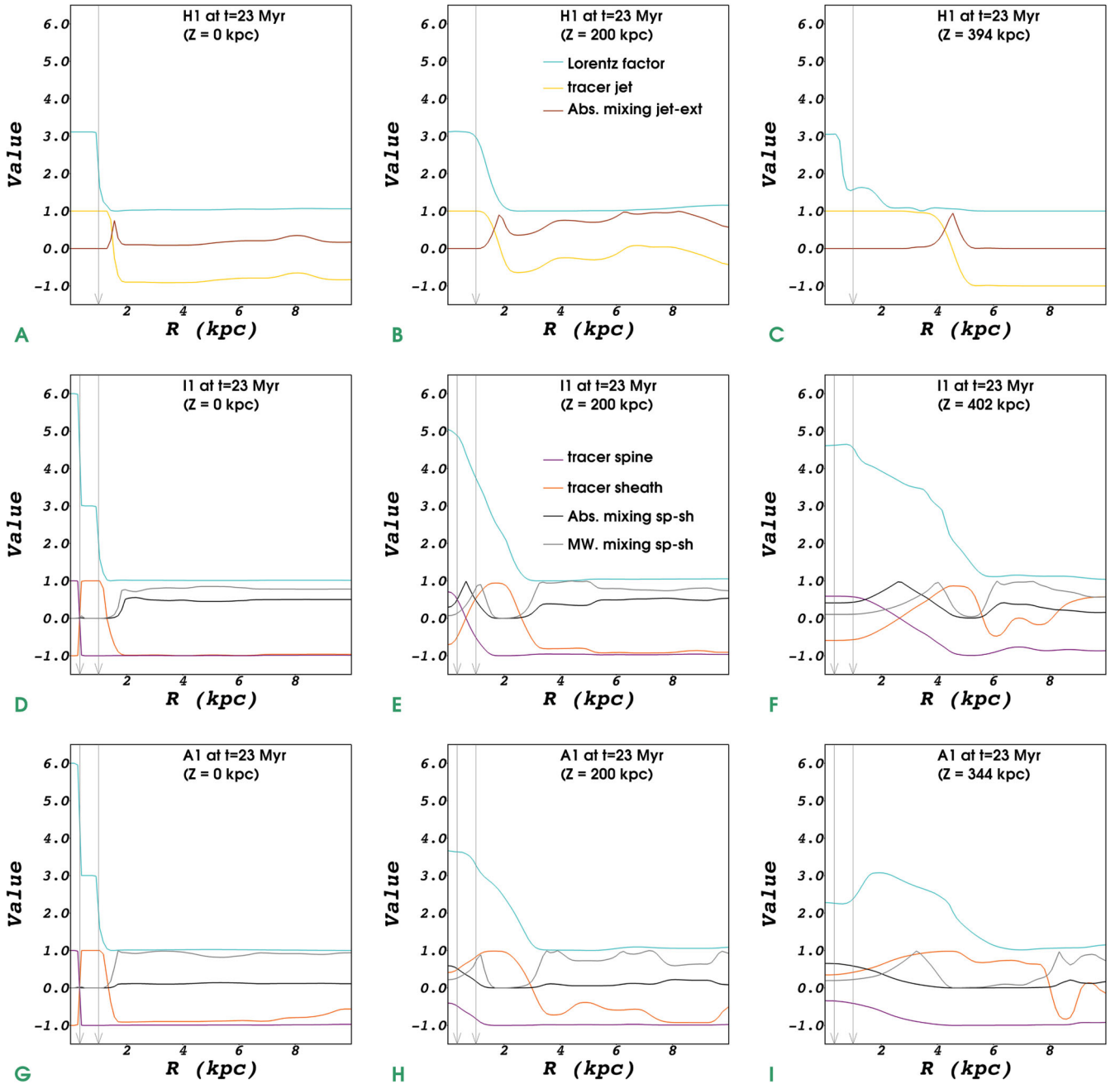
Figure 5. Radial cuts along the cylindrical radial direction at three different heights, showing Lorentz factor, tracer values and the absolute and mass-weighted mixing factor. The top row (plots A–C) shows radial cuts for model H1 . The legend shown in panel B applies to the top row, except for the Lorentz factor which applies to all plots. The middle row (plots D–F) shows model I1 . The legend shown in panel E applies to this middle row and the bottom row. The bottom row (plots G–I) shows model A1 . In the first column, a radial cut is made at the jet inlet at Z = 0 kpc. In the second column, a radial cut is shown at a distance Z = 200 kpc from jet inlet where all jets ( H1 , I1 and A1 ) have crossed three strong internal shocks. In the third column, a radial cut is shown just below the hotspot (where the effective polytropic index drops below \Gamma_{\text{eff}} \leq 1.417 ). The exact location of the hotspot for these three jet models differs. The vertical arrows in all line plots (A through I) at R = 1 kpc mark the initial jet radius. The vertical arrows at R \sim 0.3 kpc mark the initial jet spine–jet sheath interface.
