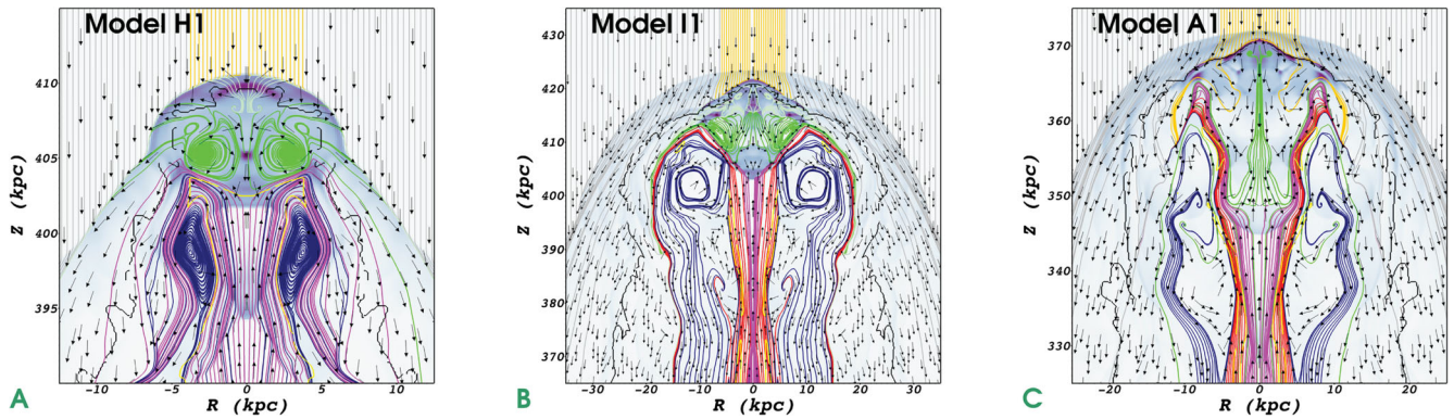
Figure 6. Close-up of the jet-head structure for the models H1 , I1 and A1 at the final time of simulation, t = 22.8 Myr. Plot A shows the homogeneous jet, B the isothermal jet and C the isochoric jet. Various regions of the flow (in the frame of the advancing Mach disc) have been depicted by different flow line colours (see Section 4.6 for a full explanation). The main features in the plots are the jet flow, the effective impact area of the ambient medium that impacts the jet, and regions of vortex formation and turbulent mixing.
