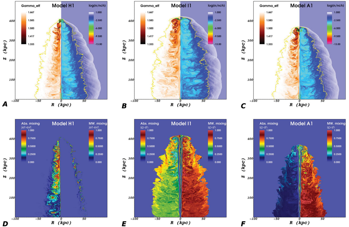
Figure 7. Contour plots of the homogeneous jet ( H1 , panels on the left-hand side), the isothermal jet ( I1 , centre panels) and the isochoric jet ( A1 , panels on the right-hand side) after 22.8 Myr. Note: the R -axis has been stretched by a factor of 2.5 in order to enhance the visibility of the actual jet behaviour. Contour plots (A–C) show the effective polytropic index \Gamma_{\text{eff}} (left-hand side of the plots) and the \log_{10} of the number density in terms of the characteristic number density n_{\text{ch}} = 10^{-3} \text{ cm}^{-3} (right-hand side of the plots). The yellow contour marks the boundary where jet material (shocked, as well as unshocked) is found. The green contour (mainly found at the jet-head) encloses relativistic gas with \Gamma_{\text{eff}} \leq 1.417 . Contour plots (D–F) show the absolute mixing ( \Delta ) on the left-hand side of the plots and the mass-weighted mixing ( \Lambda ) on the right-hand side of plots. For the homogeneous jet ( H1 ), the mixing between (shocked) jet material and shocked ambient medium (denoted as ‘ext’) is shown, as described by equations (45) and (47). For the isothermal jet ( I1 ) and the isochoric jet ( A1 ), absolute mixing \Delta_{\text{sp-sh}} and mass-weighted mixing \Lambda_{\text{sp-sh}} between (shocked, as well as unshocked) spine material and sheath material is shown, as described by equations (43) and (46).
