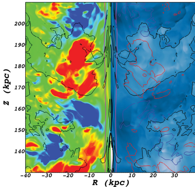
Figure 8. A close up of the isothermal ( I1 ) jet in direct contact with the surrounding cocoon. It shows the connection between internal shocks within the jet (shown by the black contours along the jet centre) and vortices in the cocoon. The pink contour from the centre bottom to the centre top of the plot marks the boundary of the jet. Left-hand panel: the red–green–blue colour scale denotes the velocity of gas in the radial direction . The red regions mark gas that is moving away from the jet and blue regions mark gas that is moving towards the jet. The red and blue contours (left- and right-hand panel) denote material moving with V_R = \pm 0.08c , respectively. Right-hand panel: the grey–blue colour scale denotes the (\log_{10}) of the gas pressure of the cocoon and jet material. Darker regions correspond to higher pressure. High-pressure regions compress the jet and cause internal shocks to emerge. These high-pressure regions correlate with gas moving towards the jet, whereas low-pressure regions correlate with gas moving away from the jet.
