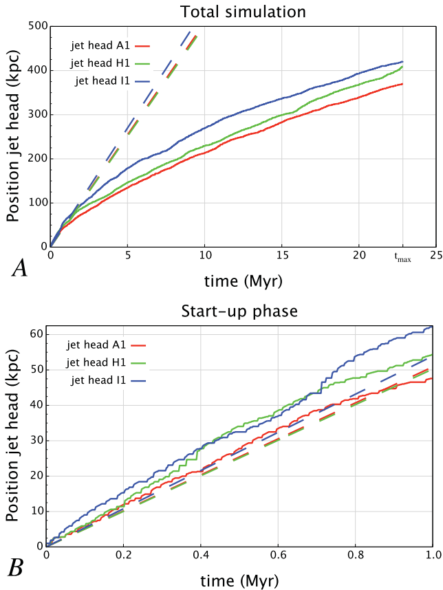
Figure 3. Jet-head propagation for all the steady jets H1 , I1 and A1 . The solid lines show the results from the simulations, the dashed lines show the analytically predicted values. Panel A shows the full duration of the simulation (up to t_{\max} = 22.8 Myr). The jet-head propagation is not constant, but decelerates after a start-up phase of \sim 1 Myr. The start-up phase of the simulations can be seen in panel B.
