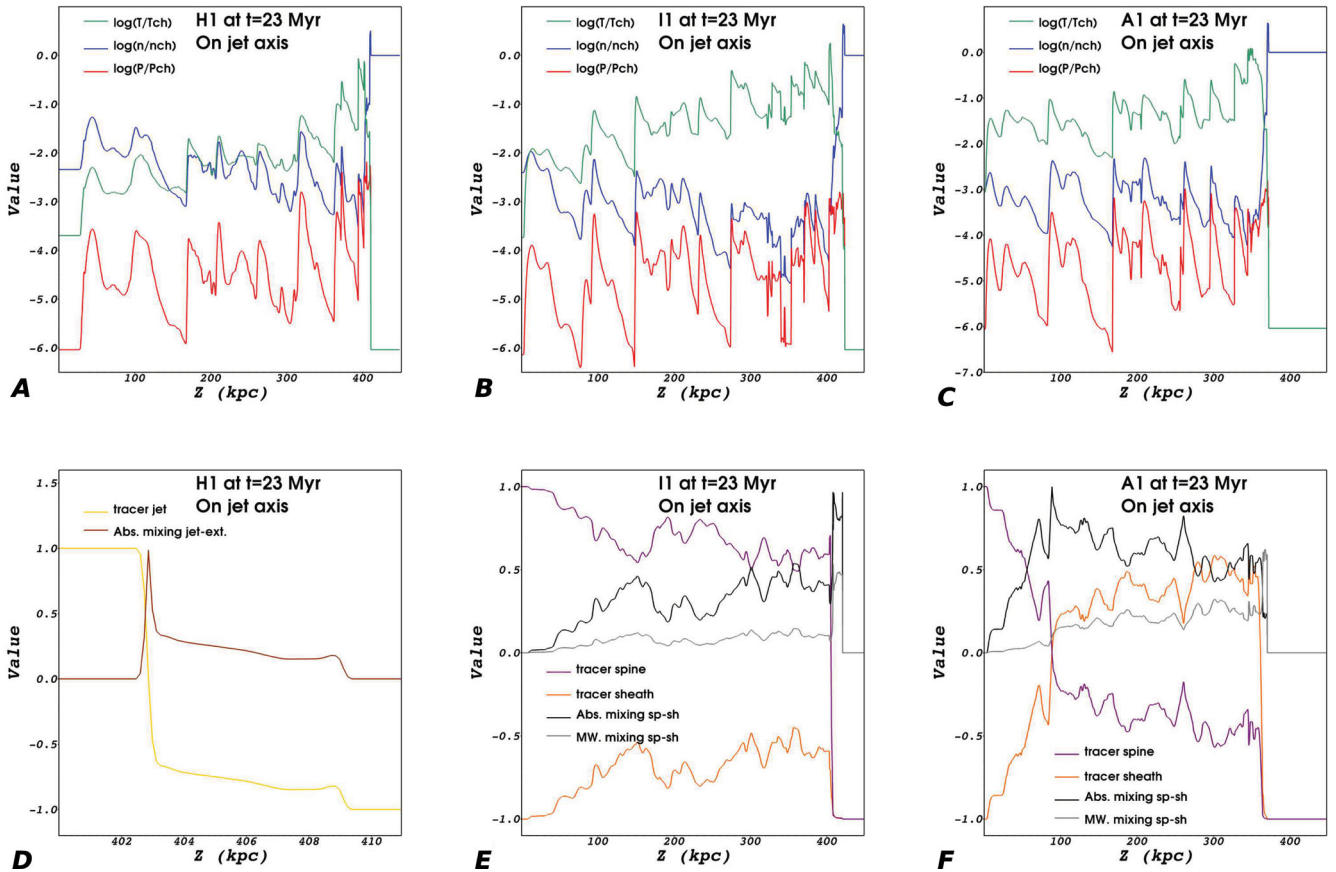
Figure 4. Cuts along the jet axis ( R = 0 kpc) for the homogeneous jet H1 (left-hand panels), the isothermal jet I1 (centre panels) and the isochoric jet A1 (right-hand panels) at t = 22.8 Myr. Top panels (plots A–C) show the \log_{10} of the number density in units of the characteristic number density n_{\text{ch}} (blue); the gas pressure in units of the characteristic pressure P_{\text{ch}} = 1.50 \times 10^{-6} erg cm ^{-3} (red); and the thermal temperature T in units of the characteristic temperature T_{\text{ch}} = 1.09 \times 10^{13} K (green). The lower panel (plots D–F) shows tracer values and absolute and mass-weighted mixing. For the homogeneous jet (plot D), only the jet-head is shown, in the range 400 \leq Z \leq 410 kpc. This is the only part along the jet axis where these variables show some variation. For the isothermal and isochoric jets (plots E and F), the tracer values of jet spine material \theta^{\text{sp}} (purple), the tracer of jet sheath material \theta^{\text{sh}} (orange), as well as the amount of internal absolute mixing (black) and the amount of internal mass-weighted mixing (grey) between jet spine and jet sheath material are shown.
