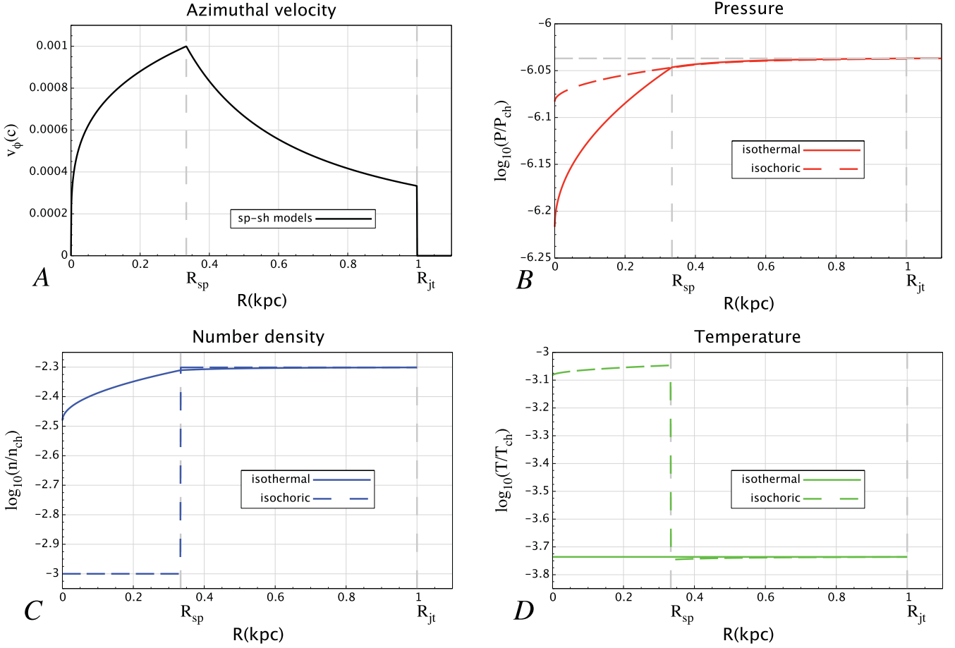
Figure 1. Initial transverse jet profiles for the isothermal jet (solid lines) and the piecewise isochoric jet (dashed lines), in case V_\phi = 1.0 \times 10^{-3}c . The cross-cuts show in black the profile of azimuthal rotation v_\phi(R) (panel A). This rotation profile has been used for both the isothermal and the isochoric jet model. In red , the \log_{10} of the pressure P in units of the characteristic pressure P_{\text{ch}} = 1.50 \times 10^{-6} \text{ erg cm}^{-3} (panel B); in blue the \log_{10} of the number density n in units of the characteristic number density n_{\text{ch}} = 10^{-3} \text{ cm}^{-3} (panel C); and in green the \log_{10} of the thermal temperature T in units of the characteristic temperature T_{\text{ch}} = 1.09 \times 10^{13} \text{ K} (panel D) of the jet. In addition, the images show the jet radius at R_{\text{jt}} = 1 \text{ kpc} and the jet spine radius at R_{\text{sp}} = R_{\text{jt}}/3 as the two vertical dashed lines. The pressure of the ambient medium is denoted by the dashed horizontal line in panel B.
