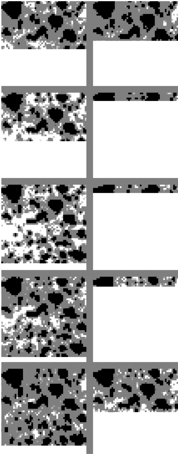
FIG. 2.—Collection of (parts of) the 10 exposures of which the 1996 February 8 image is composed, ordered chronologically downward from the top left and continuing from the top right. An object appears near the edge of the 10th frame but not in the other frames. The 10 frames are centered on this variable object at R.A. 17^{\text{h}}44^{\text{m}}37^{\text{s}}.8 and decl. -28^{\circ}45'11''.7 .
