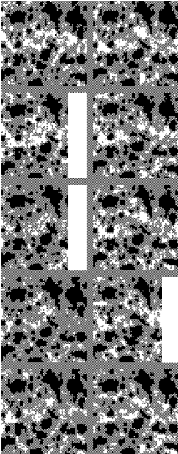
FIG. 4.—As in Fig. 2, but centered on R.A. 17^{\text{h}}44^{\text{m}}34^{\text{s}}.3 and decl. -28^{\circ}46'11.0 . Near the center of the seventh, eighth, and ninth frames, an ellipse-shaped object is seen that is not detected in the other frames.
