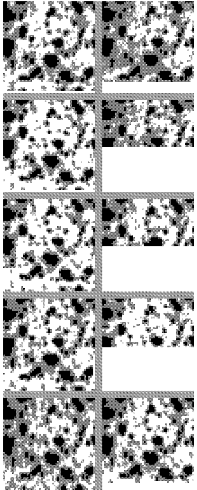
FIG. 3.—As in Fig. 2, but centered on R.A. 17^{\text{h}}44^{\text{m}}38^{\text{s}}.7 and decl. -28^{\circ}45'08''.7 . An object appears near the edge of the eighth frame but not in the other frames.
