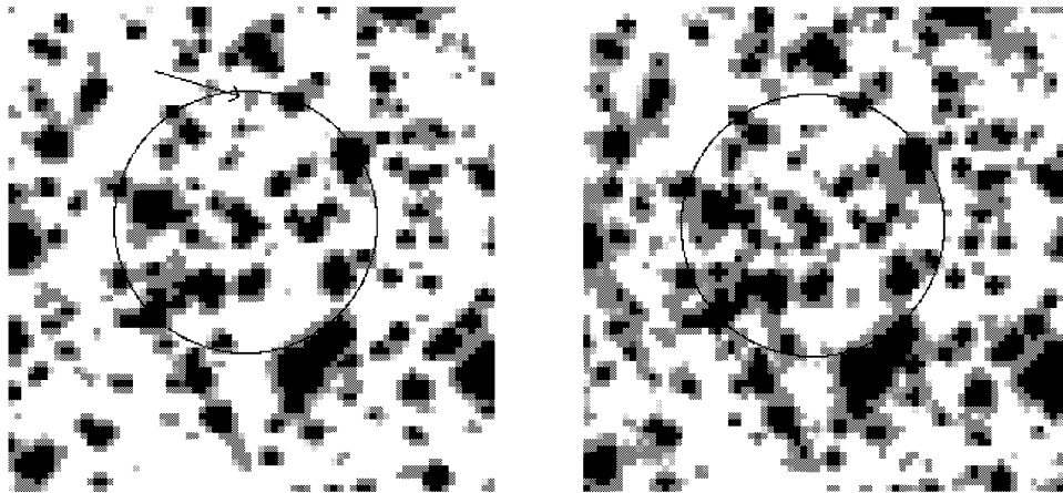
FIG. 1.—(a) Detail of a K -band image showing the 10" (radius) ROSAT error box of GRO J1744–28. This image was taken on 1996 February 8. (b) Same as (a), but image taken on 1996 March 28. The variable object is indicated.
