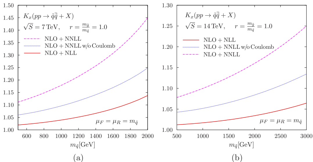
Figure 4. The K -factor with respect to the NLO cross section of the NLO+NNLL and NLO+NNLL (both with the Coulomb part \mathcal{C}^{\text{Coul},(1)} and without it) squark-antisquark cross sections for the LHC at 7 TeV (a) and 14 TeV (b). The squark and gluino masses have been taken equal and the common renormalization and factorization scale has been set equal to the squark mass.
