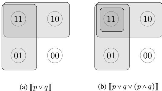
Figure 1: The proposals denoted by (1) and (3) are distinct.
