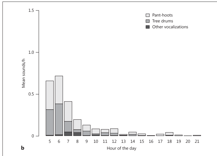
Fig. 3. Types of sound produced per hour by chimpanzees in Gangu ( a ), and all regions except Gangu ( b ) and their distribution over the course of the day.
