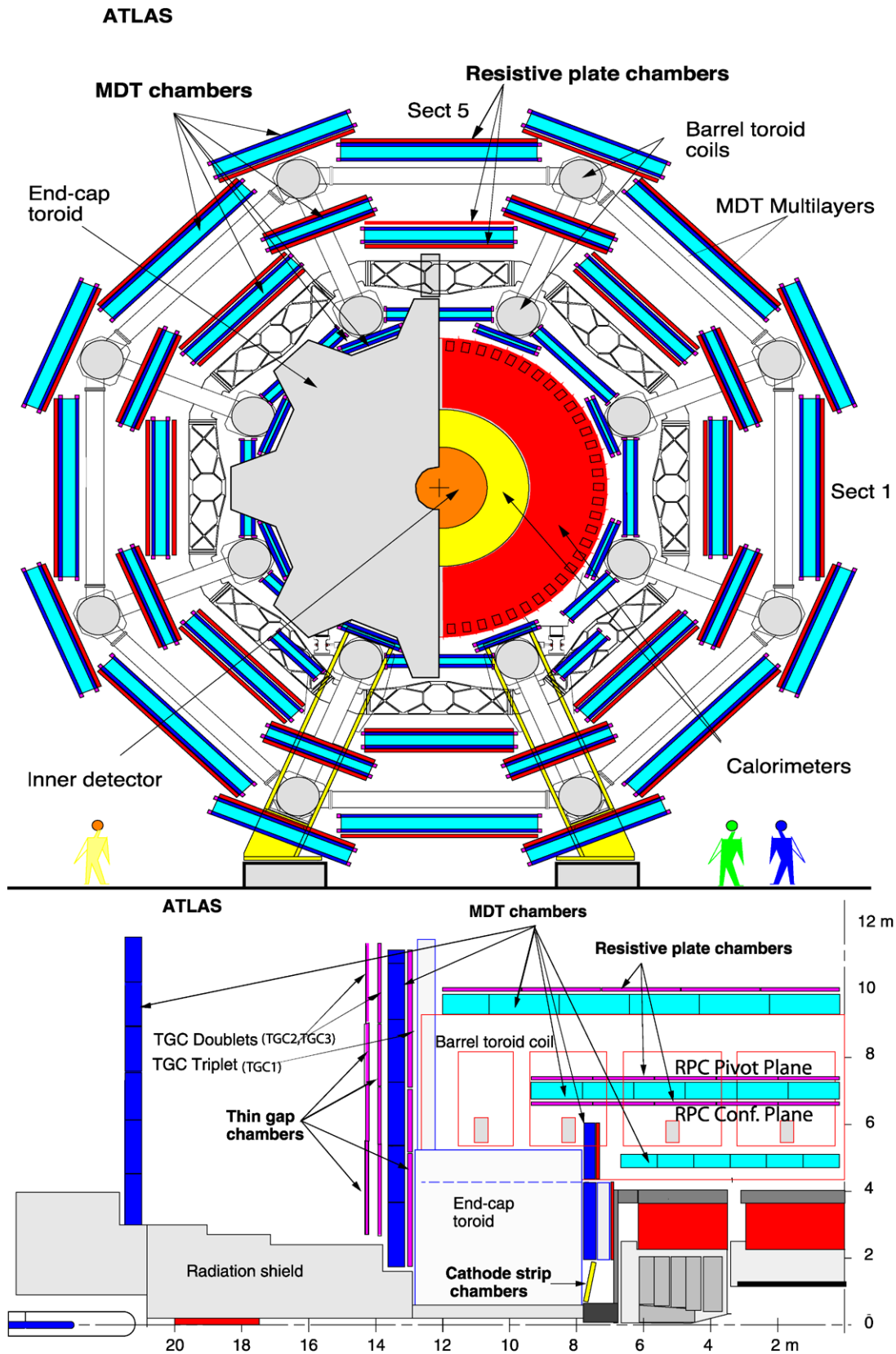
Fig. 1 Schematic view of the muon spectrometer in the x - y (top) and z - y (bottom) projections. Inner, Middle and Outer chamber stations are denoted BI, BM, BO in the barrel and EI, EM, EO in the end-cap
