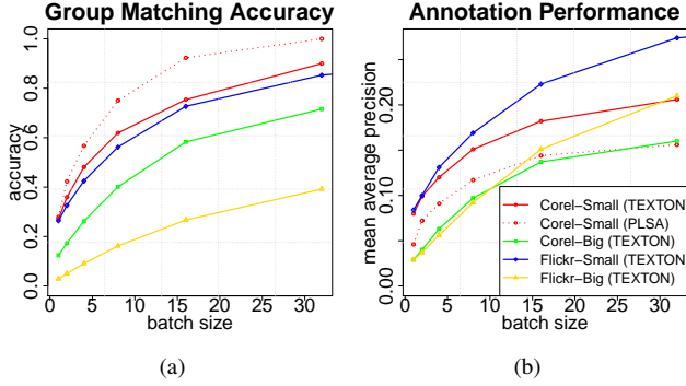
Fig. 7. Plotting (a) the accuracy of group matching and (b) annotation performance against the number of pictures in a batch. For a batch size of 1, our approach performs comparable to standard base models not using context. The more pictures we have in the context, the more reliable both group matching and overall annotation become.
