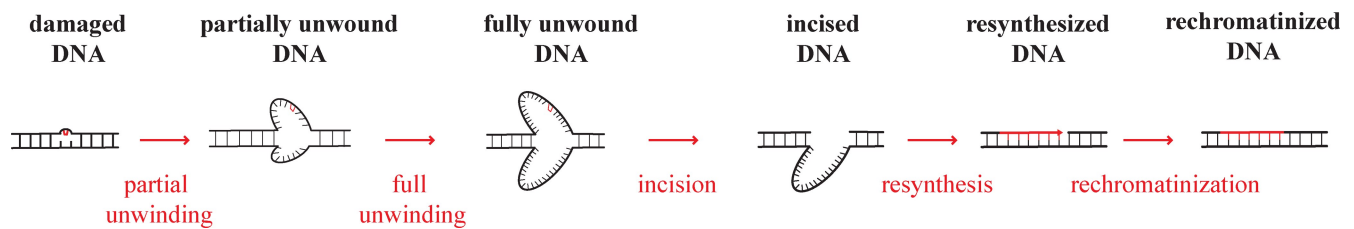
Figure 1. DNA repair intermediates for NER. The different states of the DNA substrate during NER (repair intermediates) are interconverted by a series of enzymatic reactions (red arrows).
