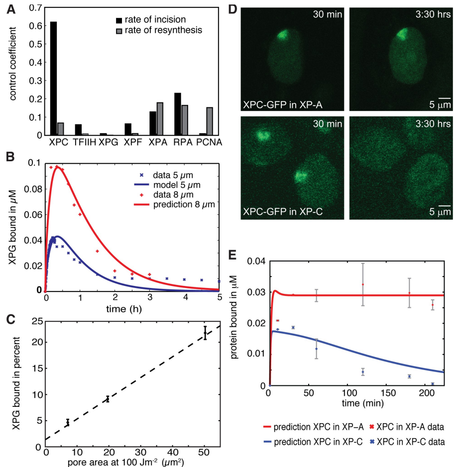
Figure 7. Capacity of NER. (A) Control of NER proteins on the rate of incision (black) and rate of DNA resynthesis (gray). Control coefficients were calculated with the following equation:
