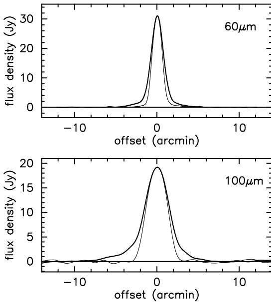
Fig. 5. Survey scan data of U Ant (thick lines) in the IRAS 60 \mu m and 100 \mu m bands. Upper and lower panels are for the 60 \mu m and 100 \mu m scans, respectively. Thin lines show the point source templates derived from the scan data of \beta Gru (M5III). The offset is negative before the passage (namely to the north-east) of the stellar position
