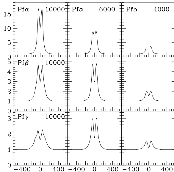
Fig. 6. The effect of a temperature gradient on on the line profiles of Pf\alpha , Pf\beta , and Pf\gamma for the standard density. The temperature in K is given in the upper right corner and is constant in each column; the line identification is given in the upper left corner and is the same in a given row
