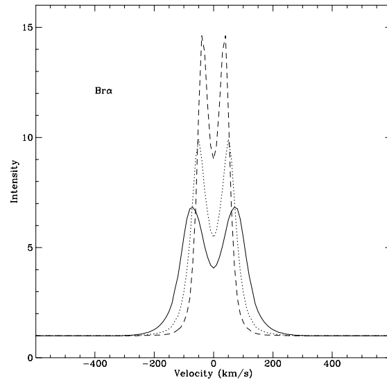
Fig. 11. The effect of the temperature on the line profile for the \text{Br}\alpha line. The surface density is 3.0 \times 10^{-12} \text{ gm/cm}^3 . The solid line is for T = 10000 \text{ K} , the dotted line for 4000 \text{ K} and the dashed line for 2000 \text{ K} . All other parameters have their standard values
