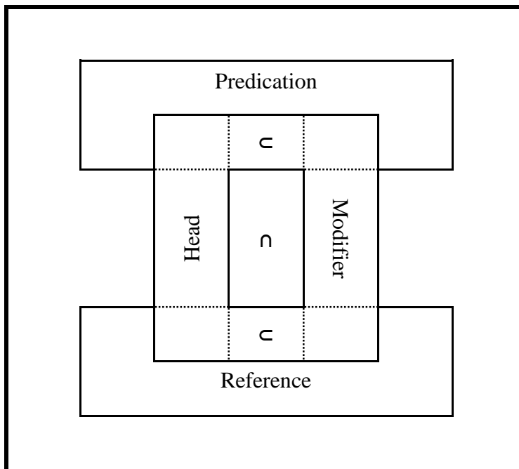
Figure 7: The implicational map of parts of speech
