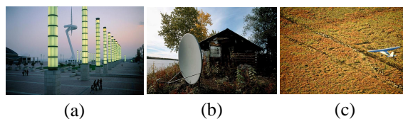
Figure 2: Typical images for three sub-models of the integrated Weibull distribution. Figure (a) corresponds to the power law sub-model, (b) and (c) show, respectively, examples for the exponential and the Gaussian sub-models.
