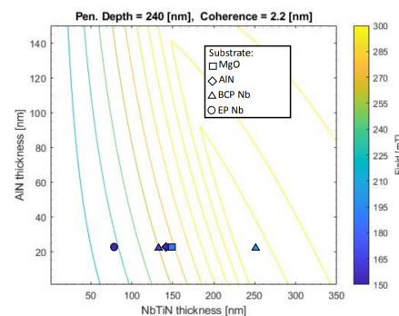
Figure 1: Theory showing the H_{c1} for SIS structures of NbTiN-AIN on Nb [2]. The calculation, for NbTiN, assumes a London penetration depth of 240 nm and a coherence length of 2.2 nm and for the Nb bulk, a London penetration depth of 40 nm. The shapes are previous SQUID and 3^{\text{rd}} harmonic measurements with the fill color corresponding to the H_{\text{fp}} of the sample.
