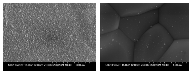
Figure 16: SEM images of the coated samples with twin axis cavity #2.
