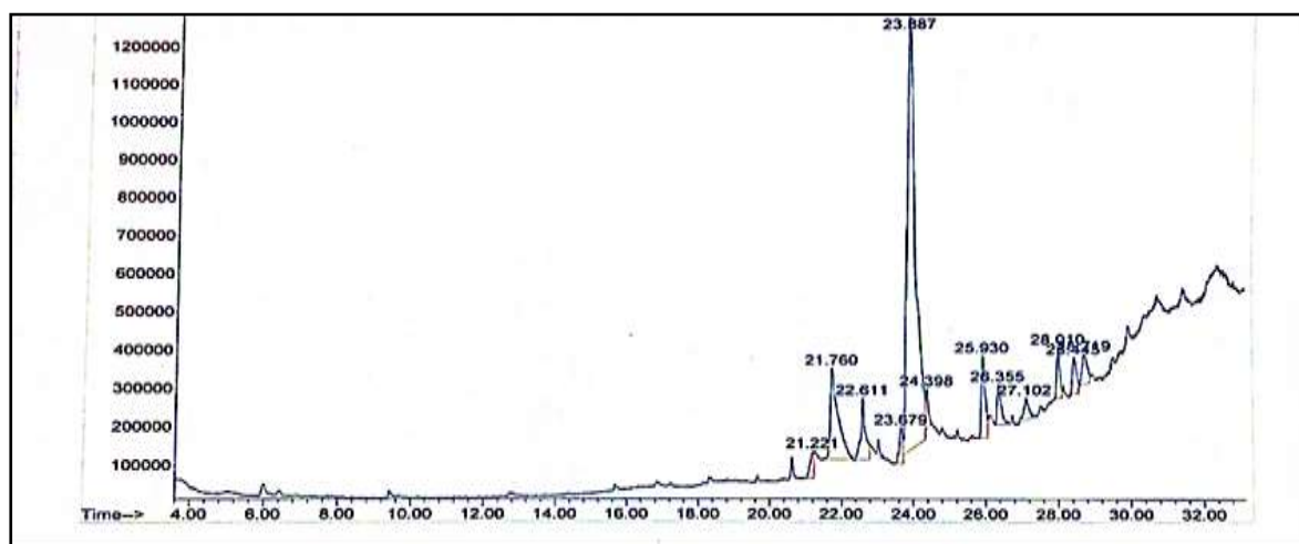
Figure 5. GC/MS chromatogram for n-hexane fraction of Agave attenuata roots
