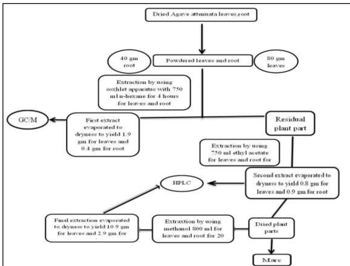
Figure 2. Extraction scheme of different phytoconstituents from Iraqi Agave attenuata
