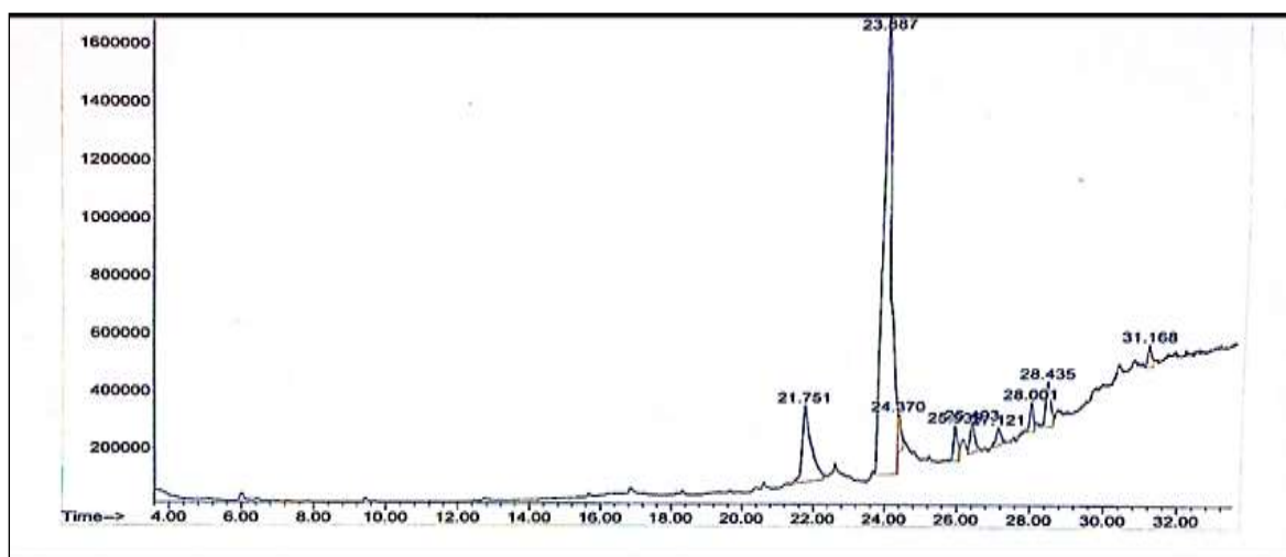
Figure 4. GC/MS chromatogram for n-hexane extract of Agave attenuata leaves.
