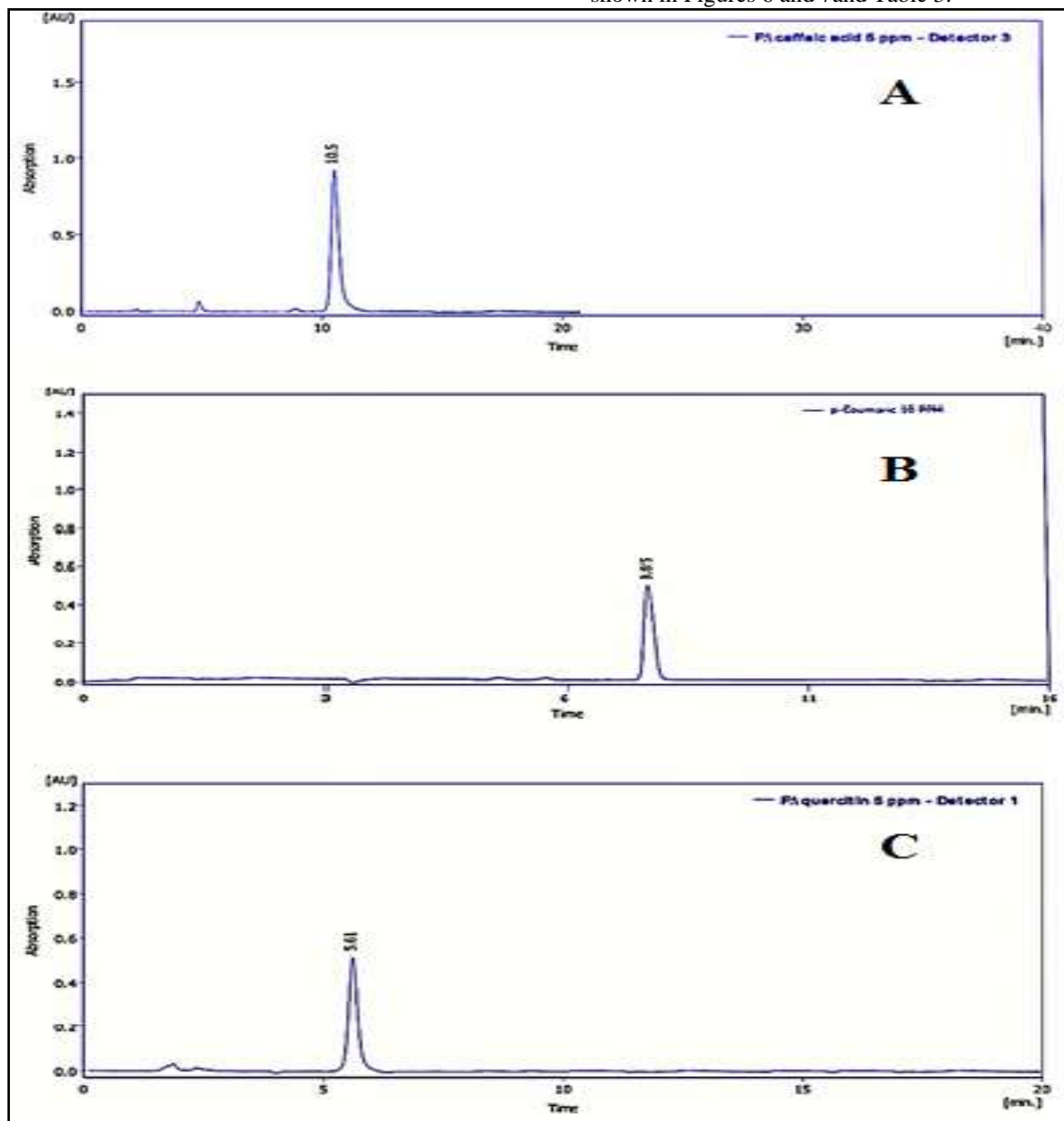
Figure 6. HPLC chromatogram for, A: caffeic acid standard, B: p-coumaric acid standard and C: quercetin standard
