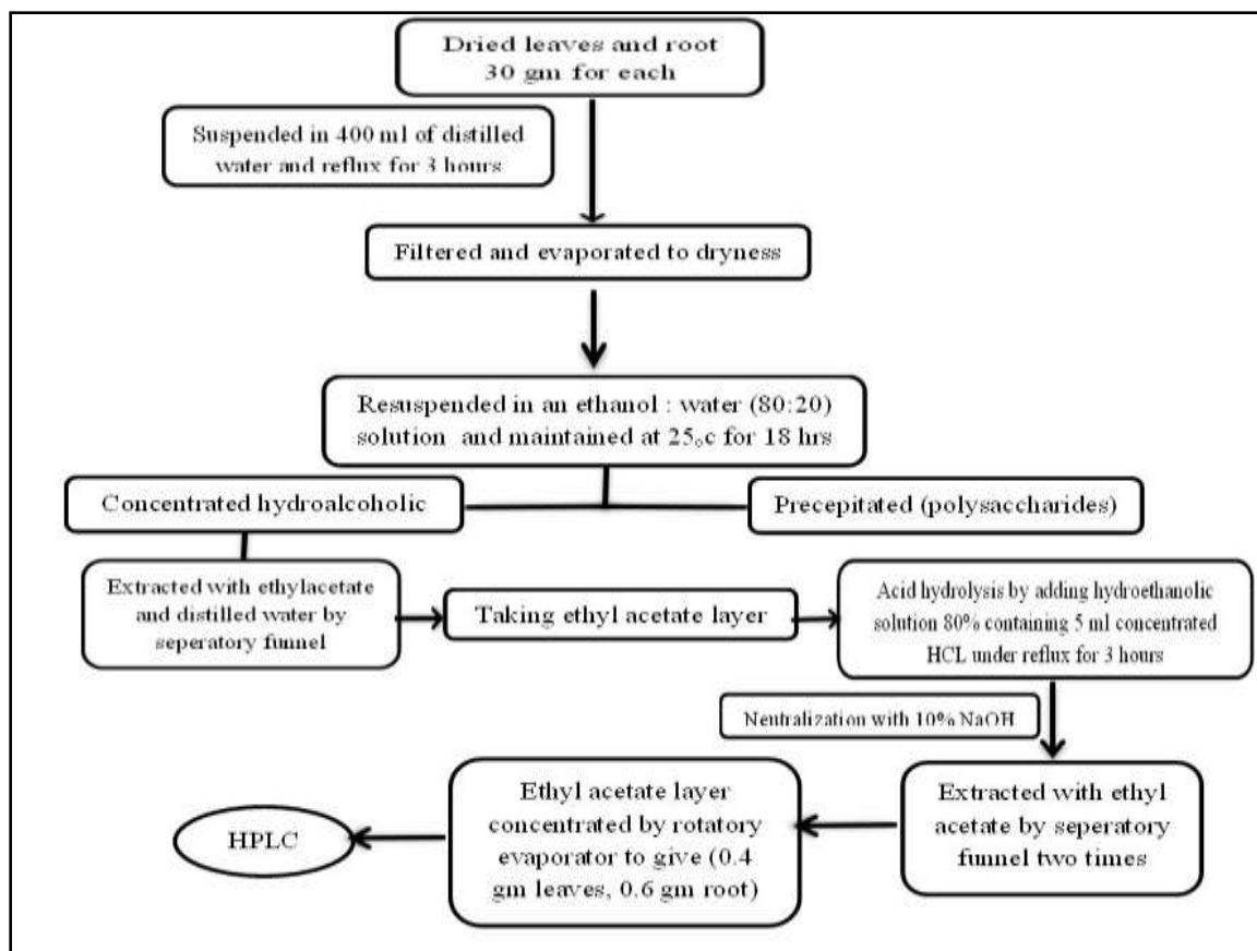
Figure 3. Extraction scheme of steroidal saponin from Iraqi Agave attenuata
