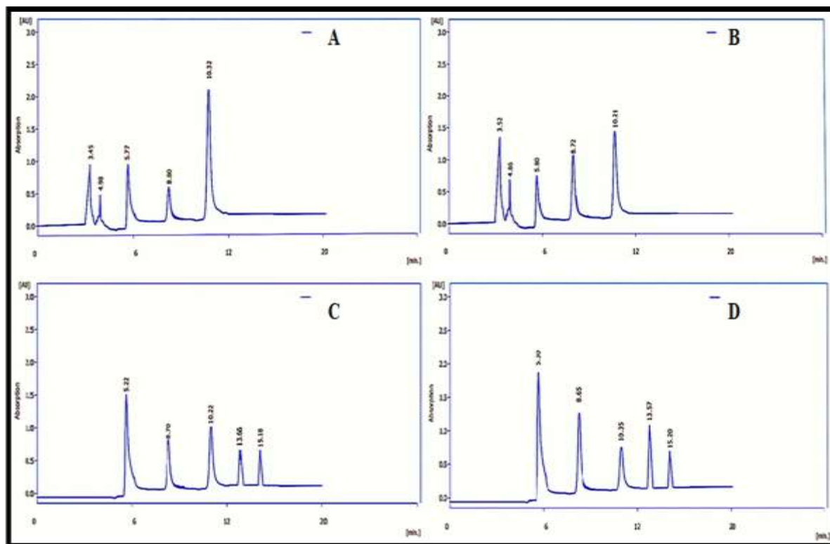
Figure 7. HPLC chromatogram of, A: ethyl acetate fraction of the leaves, B: methanol fraction of the leaves, C: ethyl acetate fraction of the roots, D: methanol fraction of the roots.
