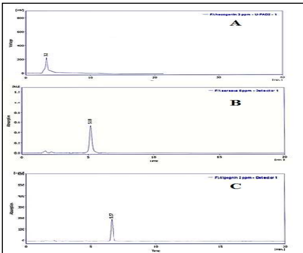
Figure 8. HPLC chromatogram for, A: Hecogenin standard, B: Sarsasapogenin standard and C: Tigogenin standard
