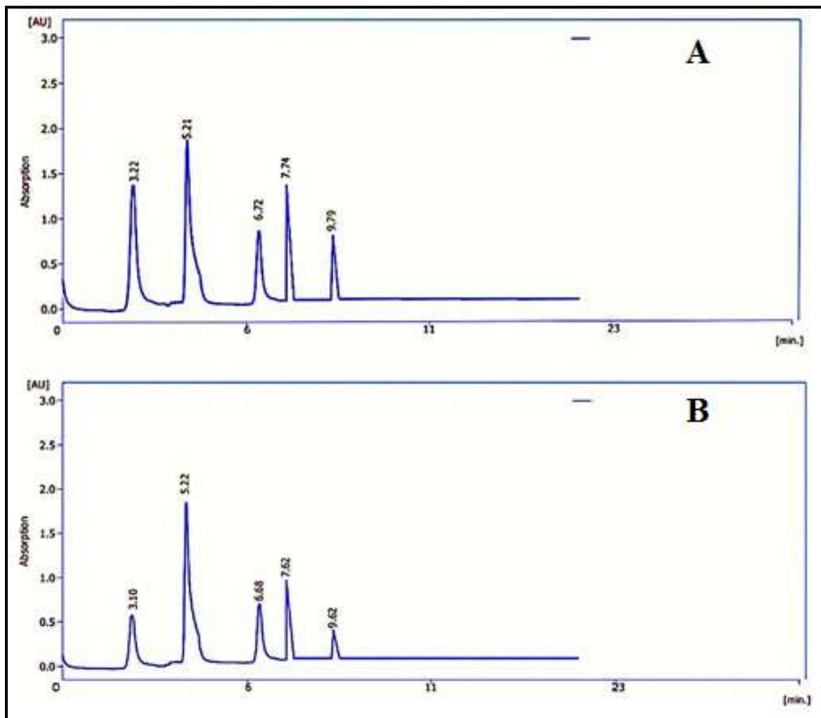
Figure 9. HPLC chromatogram of saponin fraction of the, A: Leaves and B: Roots.
