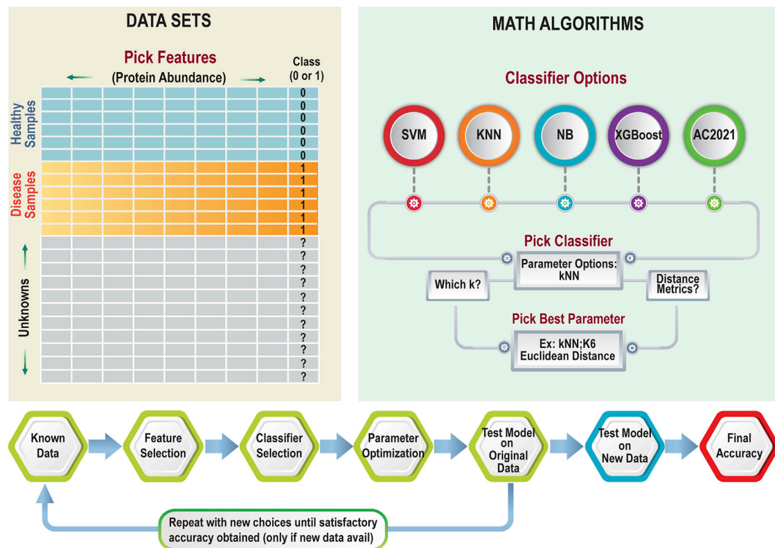
Figure 2. Required components and example work flow for supervised classification
