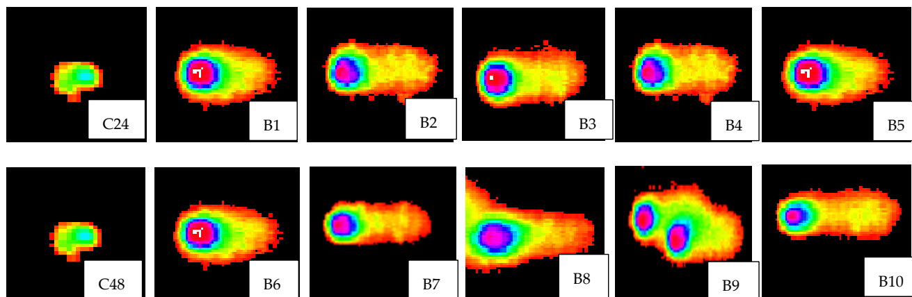
(b) Tartrazine E-102
