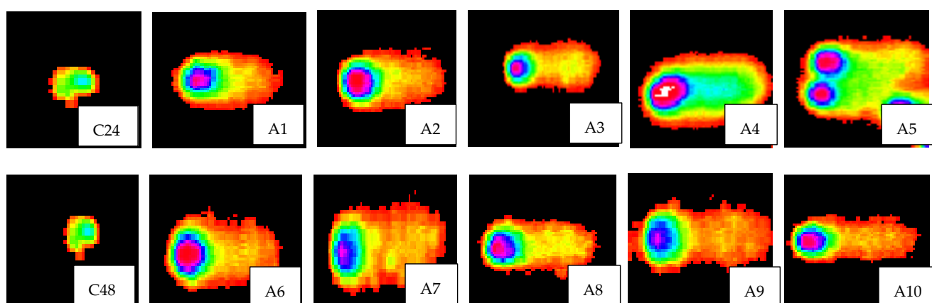
Figure 3. Interpretation of comet scores by using the comet scoring software. Images from B1 to B5 and B6 to B10, along with controls, show the comets of Azorubine E-122 at both 24 and 48 h exposure time, whereas the comets of Tartrazine E-102 are shown from T1 to T5 and T6 to T10 and Allura red AC E-129 are shown from A1 to A5 and A6 to A10 at both 24 and 48 h exposure times. Dilution concentrations were 0.25, 0.50, 0.75, 1.0 and 1.25.
