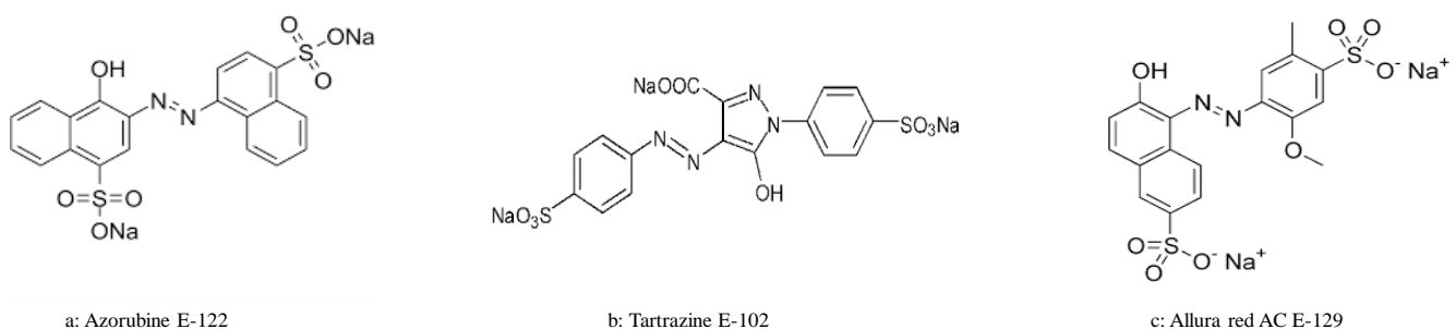
Figure 1. Chemical structures of Azorubine E-122, Tartrazine E-102 and Allura red AC E-129.
