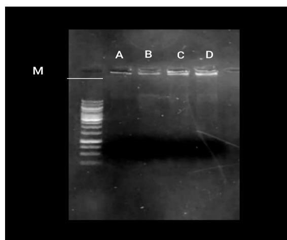
Figure 2. Quantification of genomic DNA of plant growth-promoting rhizobacteria (PGPR) on Agarose gel electrophoresis. M represents the DNA ladder of 1 kb, and the extracted genomic DNA samples of rhizobacteria are from well A to D.
