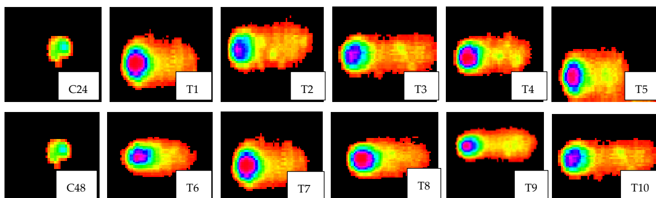
(c) Allura red AC E-129
