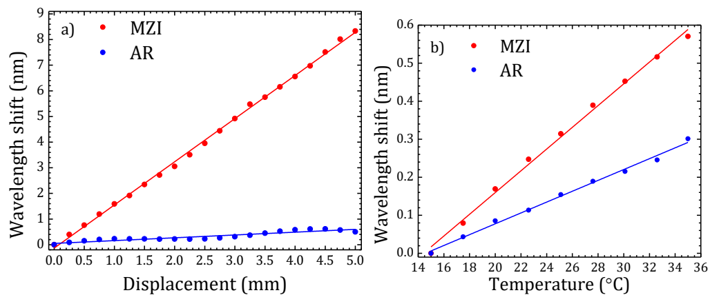
Fig. 5. Sensor response to (a) displacement and (b) temperature variations.
