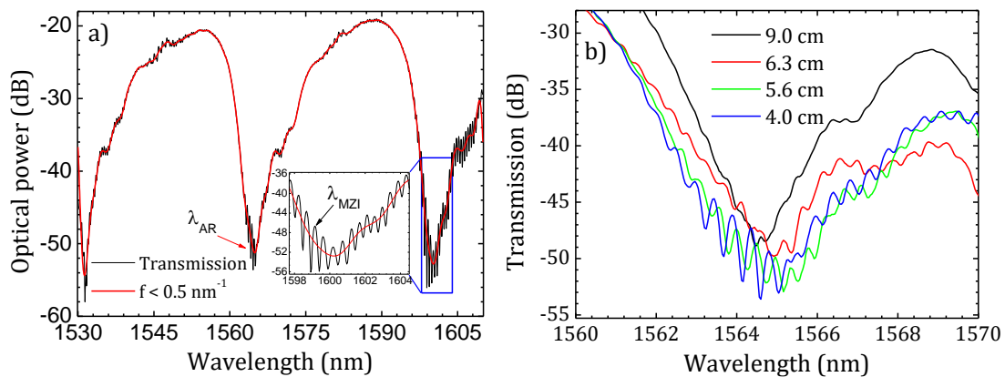
Fig. 3. (a) Transmission spectrum for a 1.2 cm sensor with 4.0 cm balloon length. Inset: Zoom-in of the spectrum in the 1598-1604 nm region. (b) Transmission spectrum for a 1.2 cm sensor with different balloon lengths in the 1560-1570 nm region.
