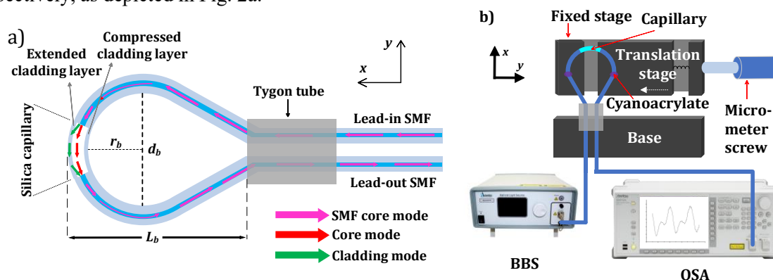
Fig. 2. (a) Schematic diagram of the balloon-like sensor. (b) Schematic diagram of the displacement setup.
