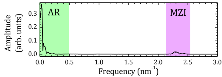
Fig. 4. FFT spectrum of the 4.0 cm balloon length sensor.
