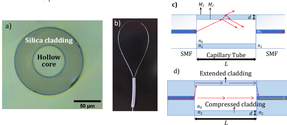
Fig. 1. (a) Microscope image of the silica capillary tube cross-section. (b) Picture of the fabricated balloon-like sensor. (c) Antiresonant reflecting optical waveguide mechanism in the capillary. (d) Mach-Zehnder interferometer schematic diagram.
