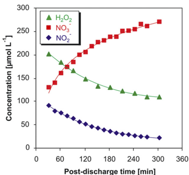
Figure 19. Evolution of the liquid phase concentration of H 2 O 2 , NO 3 - and NO 2 - after plasma treatment (pH 3.3). Reproduced from [84]. © IOP Publishing Ltd. All rights reserved.
