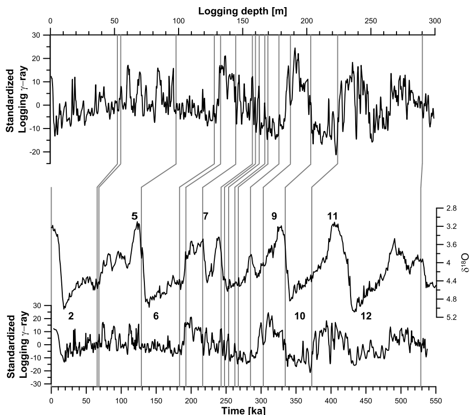
Fig. 4. Correlation of Lake Chalco's Standardized \gamma -ray depth series to the globally distributed marine benthic oxygen isotope stack ( \delta^{18}\text{O} ) and its age model (LR04 stack, Lisiecki and Raymo, 2005), and resulting age-depth model. Vertical gray lines indicate the position of tie points, and numbers point out the marine isotope stages (MIS).
