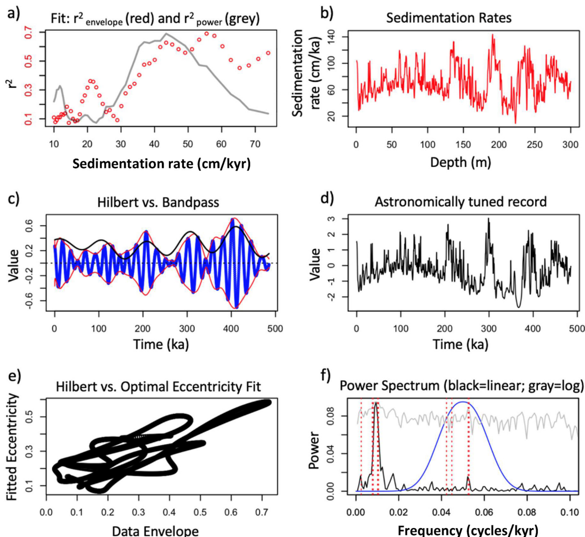
Fig. 3. TimeOpt template analysis on the detrended spectral \gamma -ray signal (SGR) for the upper 300 m of Lake Chalco. a) Squared Pearson correlation coefficient for the amplitude envelop fit ( r^2_{envelop} , red dots) and the spectral power fit ( r^2_{spectral} , gray line) at each evaluated sedimentation rate. b) timeOpt-reconstructed sedimentation rate history. c) Comparison of the band-passed precession signal (blue line), the data amplitude envelope (red line), and the timeOpt-reconstructed eccentricity model (black line). d) Astronomically-tuned stratigraphic series using the sedimentation rate history in (b). e) Crossplot of the timeOpt-reconstructed precession amplitude and the eccentricity models. f) Power spectrum of the Multitaper method (MTM) for the timeOpt derived age model and GR data using the average sedimentation rate of 43.5 cm/kyr. Black line: linear spectrum; gray line: log spectrum. The blue line indicates the bandpass filter for evaluation of the precession amplitude envelope. Vertical dashed red lines indicate the eccentricity and precession target periods. (For interpretation of the references to color in this figure legend, the reader is referred to the Web version of this article.)
