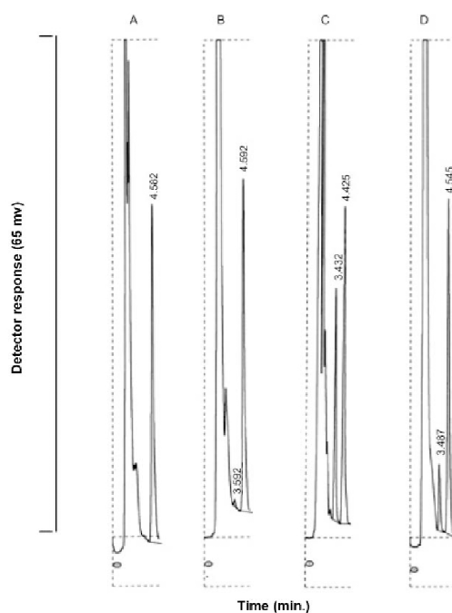
Figure 1. Typical chromatograms obtained from an extract of (A) human blank serum spiked with phenytoin as the I.S., (B) human blank serum spiked with 0.05 \mu\text{g/ml} CCA and phenytoin as the I.S., (C and D) serum samples obtained at 6 and 12 h after a single oral dose of 150 mg clopidogrel from a healthy volunteer containing 1.06 and 0.30 \mu\text{g/ml} of CCA, respectively. Peaks eluted at 3.4 and 4.5 min. correspond to CCA and the I.S., respectively.
