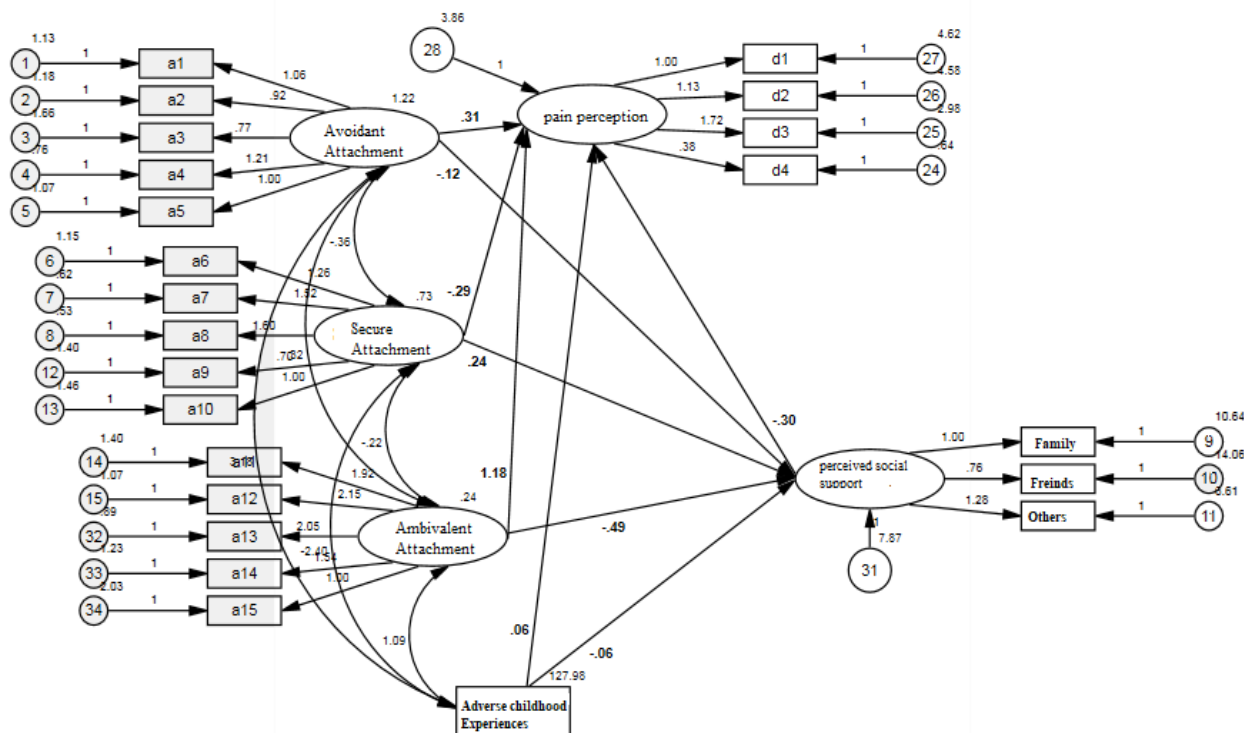
Figure 1. Structural model and its parameters using non-standard data (B).
