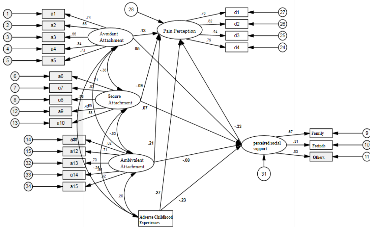
Figure 2. Structural model and its parameters using standard data (β).
