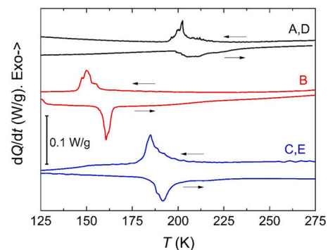
Fig. 1. DSC thermograms of different \text{Ni}_{51.5}\text{Fe}_{21.5}\text{Ga}_{27.0} samples: samples A and D, black line; sample B, red line; sample C and E, blue line. (For interpretation of the references to color in this figure legend, the reader is referred to the Web version of this article.)
