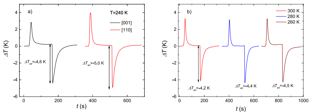
Fig. 9. Temperature change as function of time a) for samples C and E at T = 240 K, and b) for sample C at T = 260 K, 280 K and 300 K.
